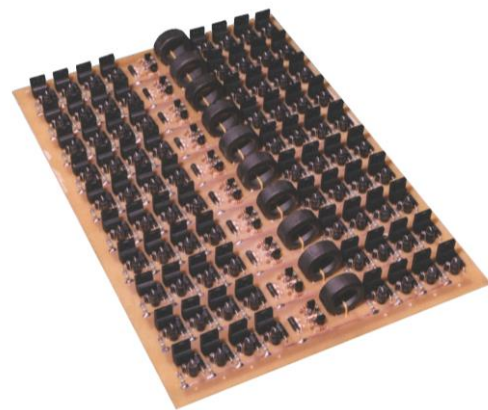
Figure 5 : MOS matrix photograph
