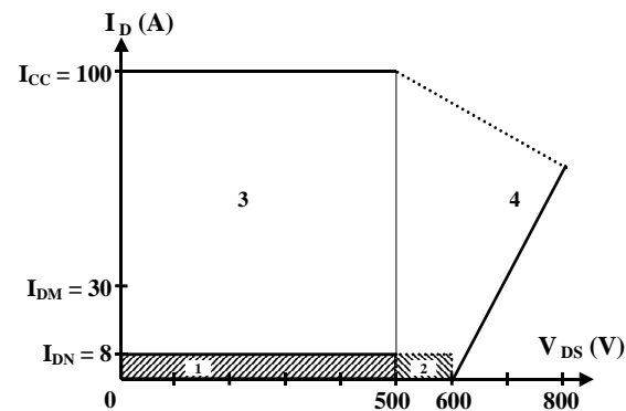
Figure 11 : MOSFET safety area
