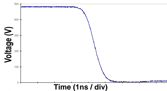
Figure 7 : Nanosecond voltage fall time
