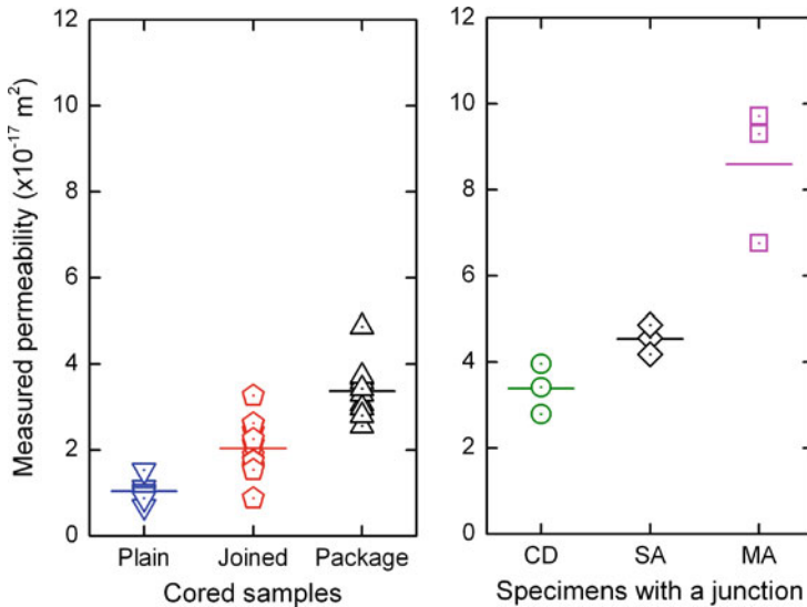
(a) Permeability of the cored samples (A = samples cored from plain specimens; B = samples cored from joined specimens; C = samples cored from the real package) (b) Permeability of the joined specimens (CD = Chemical Deactivation; SA = Strong Abrasion; MA = Medium Abrasion)
