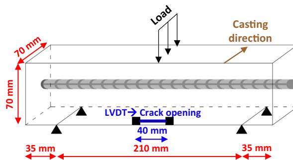
Fig. 1. Three-point bending test on 70 × 70 × 280 mm specimen.
