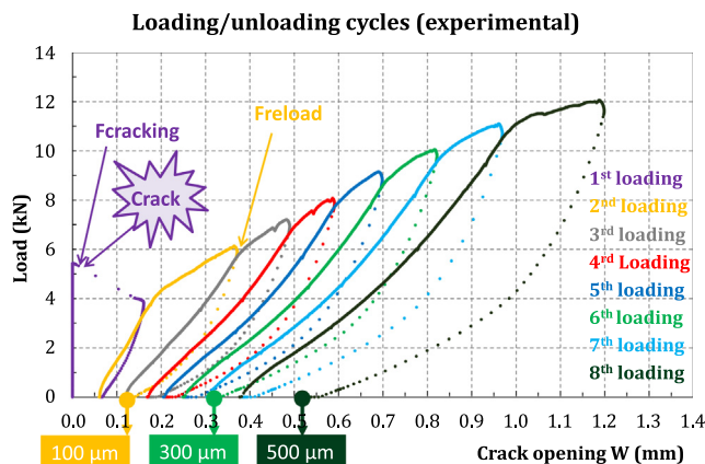
Fig. 2. Range of residual crack openings obtained by the three point bending test.
