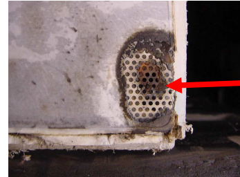
Figure 10: degradation of the separators, follow-up of fusion.
