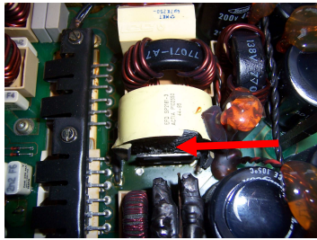
Figure 9: sight of the accused condenser.
