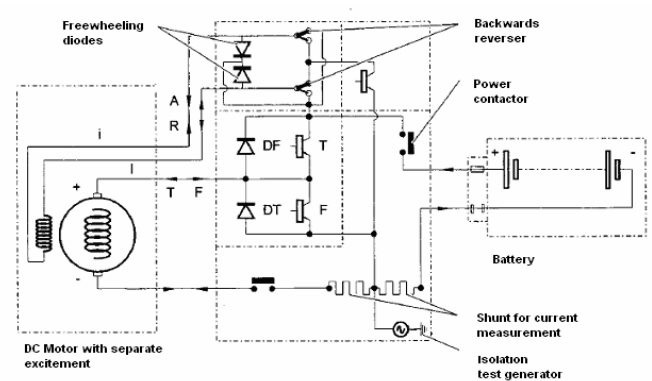
Figure 6: synoptic diagram of the converter
