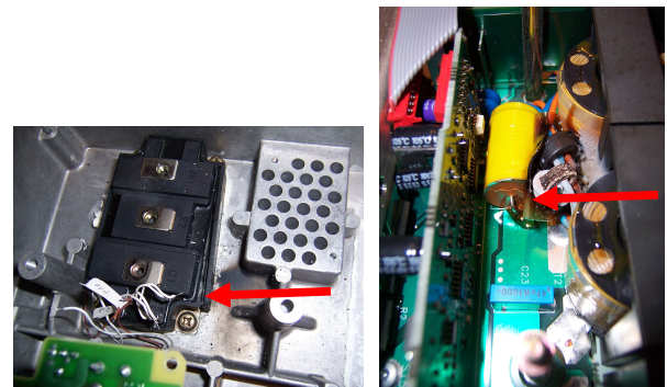
Figure 7: module IGBT destroyed Figure 8: condenser polypropylene having overheated until its destruction.
