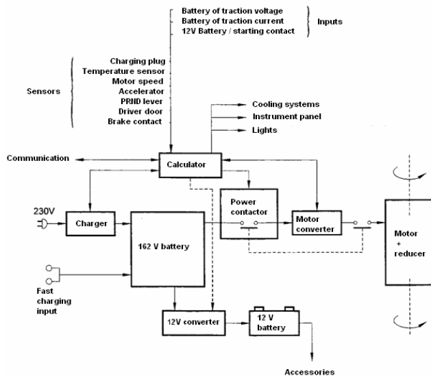
Figure 3: diagram of architecture of electronic unit for Berlingo/Partner.
