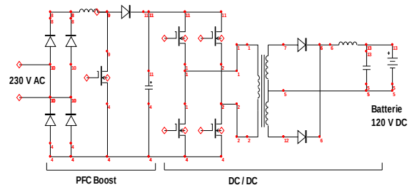
Figure 5: synoptic diagram of the battery charger of traction.
