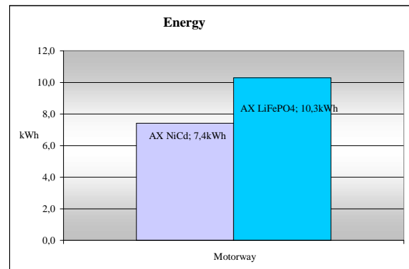
Figure 2: front pack
