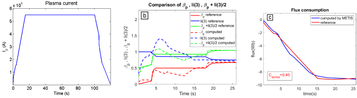
Figure 5 –First step of the simulation. (a) Plasma current time behavior taken from Ref. [21] and used as input parameter in METIS. (b) li(3) , \beta_p and li/2+\beta_p profiles computed by METIS compared with the same quantities of the simulations of Ref. [21] (used for the FEEQS-TOSCA benchmark and labelled as “reference”). (c) Comparison between the flux consumption computed by METIS and the reference one.
