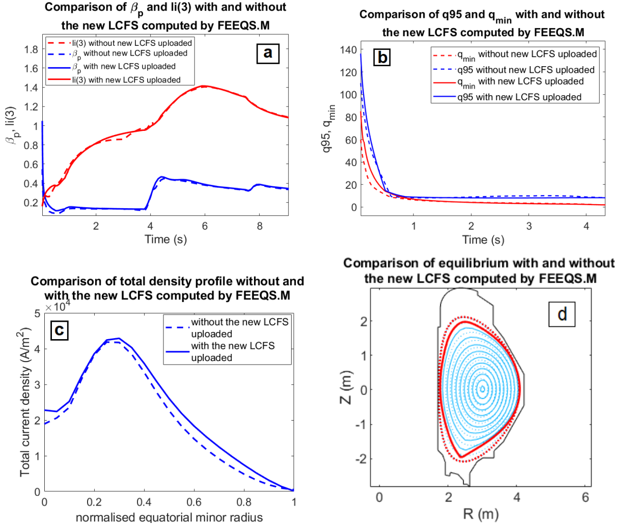
Figure 7 – Third step of simulation. (a) Comparison between \beta_p and li(3) calculated with and without the uploaded LCFS computed by FEEQS as solution of the free-boundary equilibrium problem. (b) q_{95} and q_{min} comparison between first calculation and uploaded LCFS calculation. (c) differences in behaviors of the current density profiles computed at time=3.582 s by METIS in both cases. The abscissa is the normalized Lao coordinate (normalized equatorial minor radius) [14]. (d) Comparison between equilibria with the LCFS given in METIS by points and the one computed by FEEQS at time=3.582.
