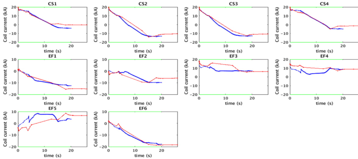
Figure 6 – Second step of the simulation. Red lines: coils currents computed by FEEQS without METIS in the loop for the ramp-up phase. Blue lines: coils currents computed by FEEQS coupled with METIS.
