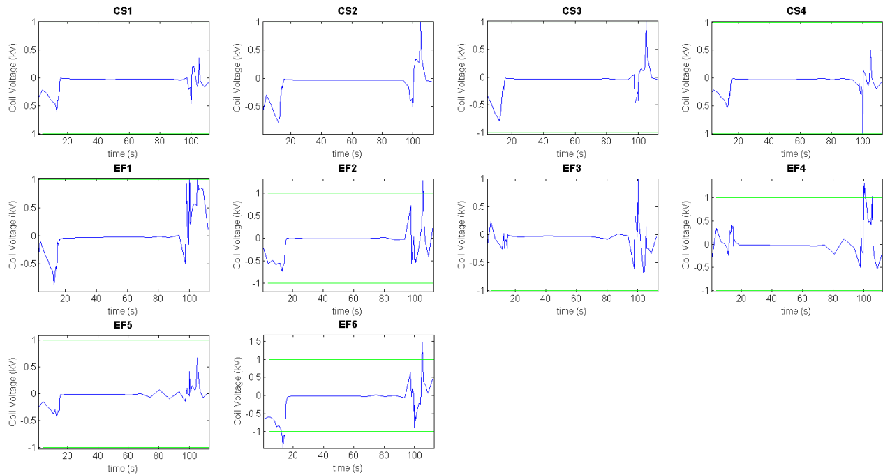
Figure 9 – coil voltage computed by FEEQS. The green lines represent the upper and the lower limits on each coil voltage. The first peaks are due to the H-mode transition, while the second peaks are due to the loss of the H-mode. During the flat-top phase all the voltages applied on the coils lie between the limits. Some singular points marginally exceed the limits.
