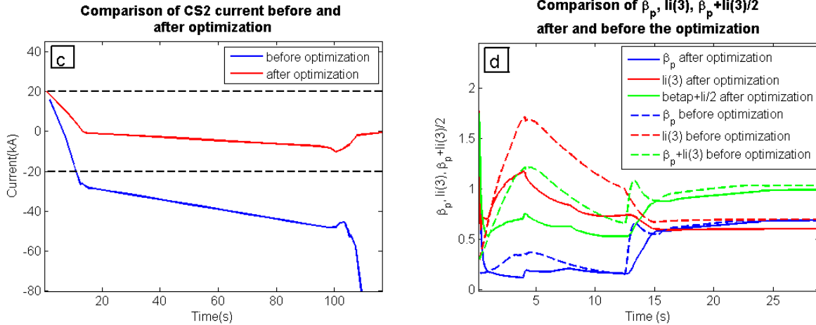
Figure 8 – (a) The waveform of the ECRH power adjusted in order to avoid the first disruption of the plasma connected to the x-point formation (at 4.09 s). (b) The waveforms of N-NBI and P-NBI powers adjusted in order to assist the H-mode transition (12.89 s). (c) The CS2 current computed for the non-optimized case and after optimization. The dashed-lines correspond to the technological coils limit. (d) \beta_p , li(3) and \beta_p + li(3)/2 computed after and before the optimization.
