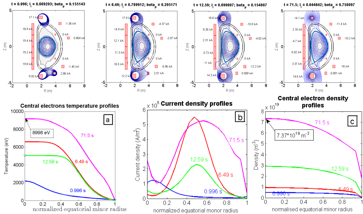
Figure 10 – Top: four plasma equilibria computed by FEEQS. From left to right the equilibrium corresponds to the time just before the x-point formation, the time after the x-point formation, the H-mode transition and a generic time during the flat-top. Bottom: The central electron temperature (a), current density (b) and density (c) profiles corresponding to the four equilibria shown in the top panels. x is the normalized Lao coordinate (normalized equatorial minor radius) [14].
