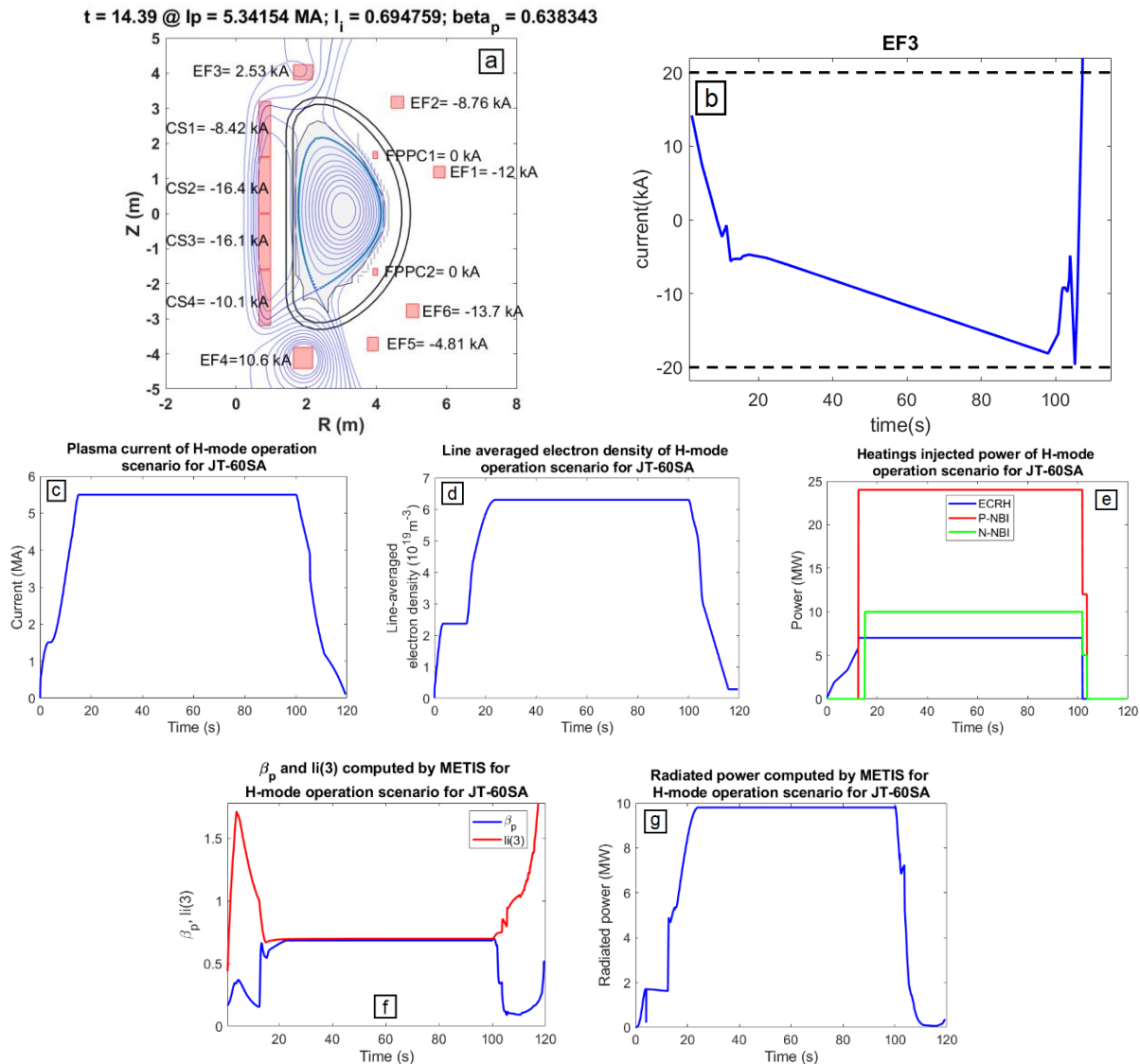
Figure 2 – FEEQS computation for the reference H-mode operation scenario of JT-60SA. (a) values of coils current computed by FEEQS for the time=14.39s and a given LCFS. Also, the value of the plasma current, li(3) and \beta_p are computed at time=14.39 s. Note: CS indicates the central solenoid coils, EF the equilibrium field coils, FPPC the fast plasma position control coils. (b) Time behavior of EF3 coil current. Dashed-lines correspond to the operational coils limit given to FEEQS as input parameters. (c-g): Time traces of the main parameters of H-mode operation scenario for JT-60SA. Plasma current (c), line averaged electron density (d), ECRH and NBIs injected power (e), li(3) and \beta_p (f) and the radiated power (g).
