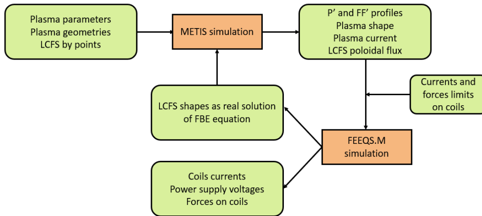
Figure 4 – Workflow combining METIS and FEEQS. In the case of the present simulations, METIS is run twice. In the first run, the LCFS is given by points; in the second run, the LCFS is computed and the full solution of the free-boundary equilibrium equation obtained by FEEQS is used.
