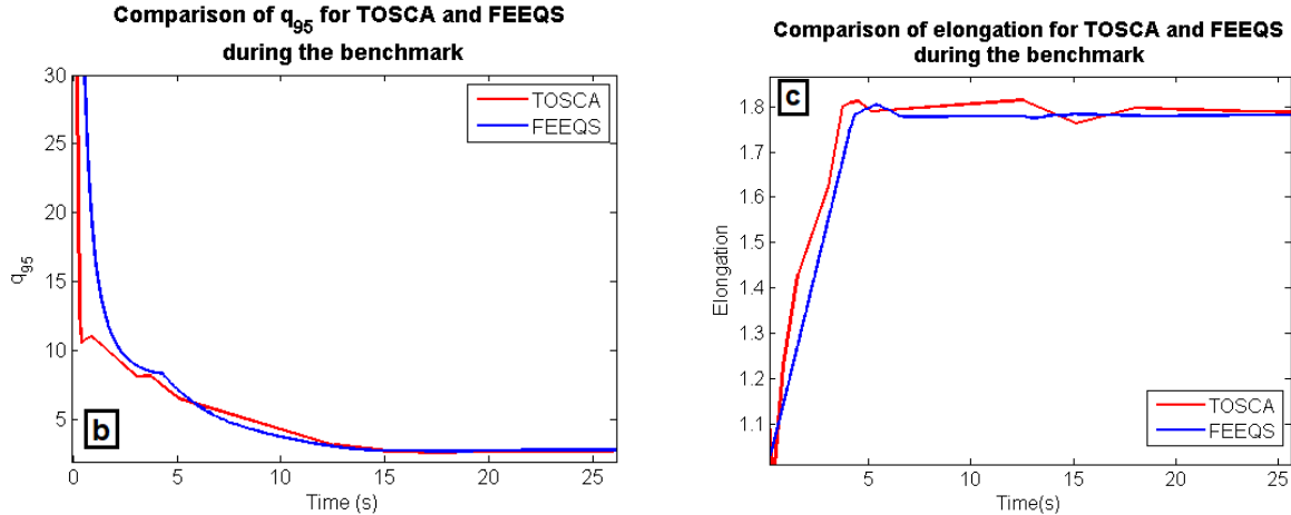
Figure 3 – (a) Comparison between coil currents from FEEQS and TOSCA for the whole discharges. CS2 current is set to the values taken from TOSCA and all of the other currents are computed using FEEQS. (b) Comparison between q_{95} from FEEQS and TOSCA for the first 25 s of the discharge. (c) Comparison between elongation from FEEQS and TOSCA for the first 25 s of the discharge.
