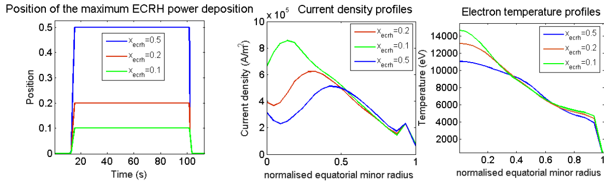
Figure 1. (a) ECRH radial power deposition positions used as input parameters in METIS for three different simulations of the standard H-mode operation scenario of JT-60SA. (b) Impact of the variation of the radial deposition on the total current density profiles computed by METIS. (c) Impact of the variation of the radial deposition on the electron temperature profile computed by METIS. The abscissa is the normalized Lao coordinate (normalized equatorial minor radius) [14]
