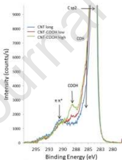
Figure 3: Normalised C-1s spectrum of CNT-COOH-high, CNT-COOH-low and raw sample. The graph shows the chemical contribution of oxygen on the C1s
