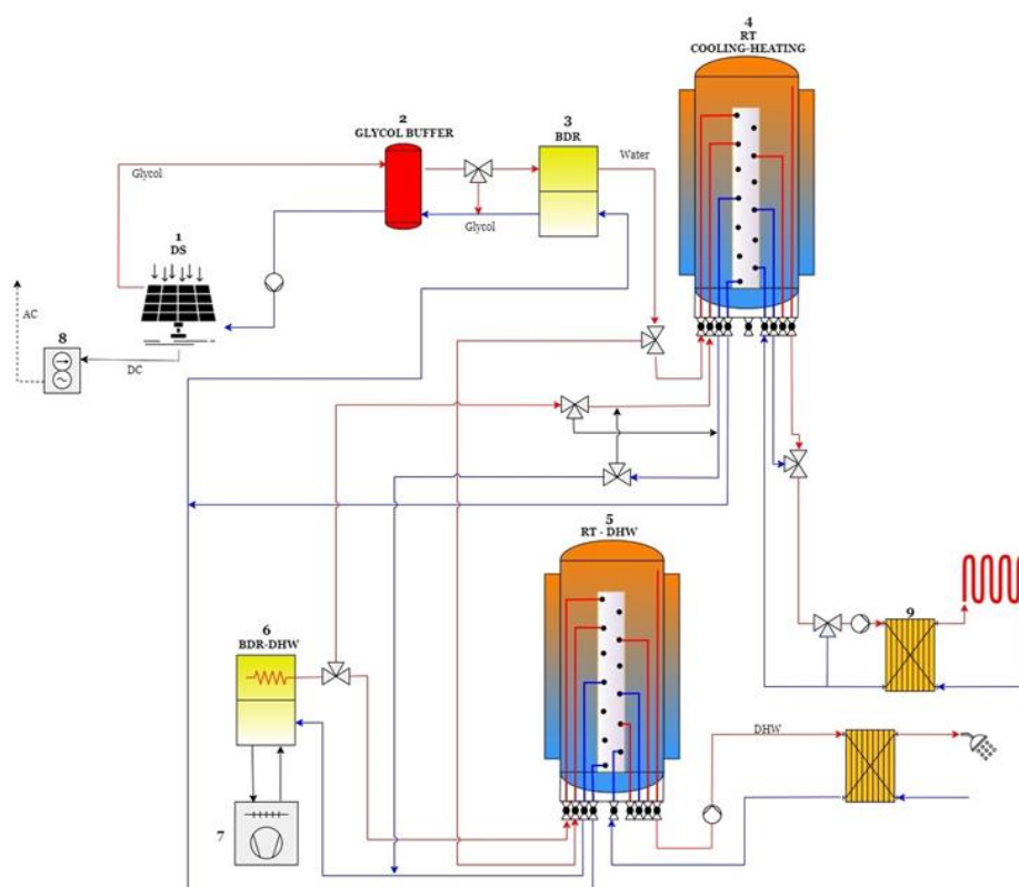
Fig. 4 Integration between existing system and SunHorizon TP4
