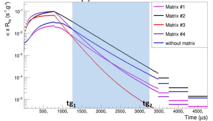
Fig. 7. Evolution of \epsilon \times R_{\text{fis}}(t) in active neutron interrogation of ^{235}\text{U} homogeneously distributed in different matrices. The blue area represents the time gate for induced-fission prompt neutron counting (useful signal).
