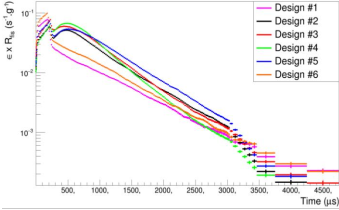
Fig. 5. Evolution of \epsilon \times R_{fis} after the 200 \mu s generator pulse, for 1 g of ^{235}U homogeneously distributed in an empty 200 L drum (without waste matrix).
