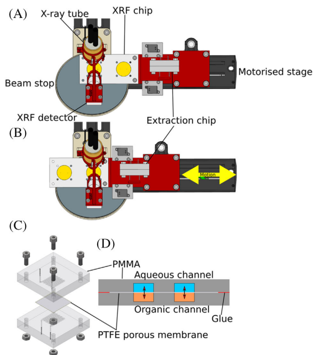
FIGURE 1 A–B, Top view of the apparatus used for the extraction and XRF experiment: The motorised stage moves both the XRF and extraction chip. The sketches show the positions that measure either the aqueous or the organic channel. C, Exploded view of the extraction chip (Reprinted from ref. [20] Copyright 2019, with permission from Elsevier) D, Cross-sectional view of the extraction chip, extraction occurs at the interface through the porous membrane. E, A picture of the whole microfluidic platform with the outer chamber doors opened
