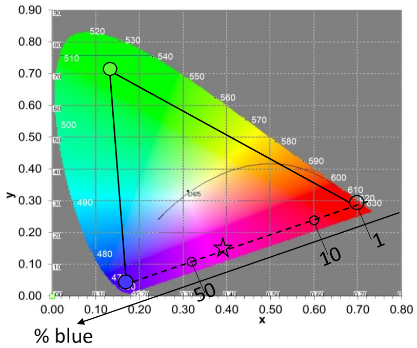
Fig. S2. Color gamut (star) of light emitted by the 4 μm-thick red-pixel of Fig.8.
