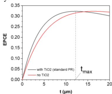
Fig. 9. (a) Evolution of EPCE (t) of red conversion layers with TiO 2 (5 wt%) and without TiO 2 . Calculation was done using data of Fig. 5 and assuming -25% on absorption without TiO 2 .
