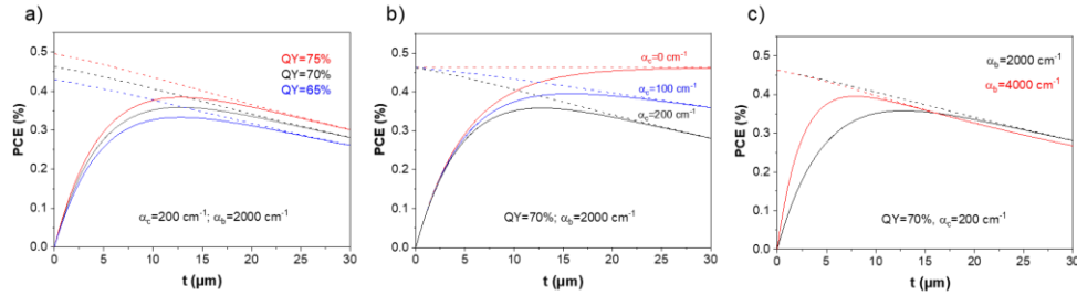
Fig. 3. Impact of model parameters on the IPCE (dashed lines) and EPCE (solid lines) functions: (a) QY , (b) \alpha_c and (c) \alpha_b . The wavelengths of excitation and emission are \lambda_b = 452 nm and \lambda_c = 650 nm.
