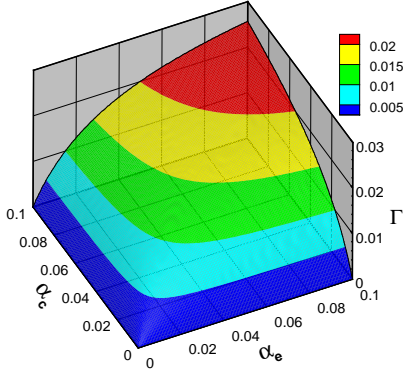
Figure 21: Instability boundary for the single branch PHP with imposed temperatures in evaporator and condenser in the parameter space (\alpha_c, \alpha_e, \Gamma) [135]. The boundary is presented as a surface which is the dependence of \Gamma on \alpha_c and \alpha_e . The oscillations can develop for the points below the surface.
