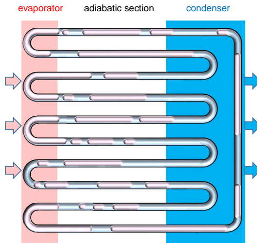
Fig. 1. Schematic representation of the pulsating heat pipe (PHP). The heated (evaporator) sections of the tube are those inside the red rectangle, while the cooled sections (condenser) are inside the blue rectangle. The tube sections in between are adiabatic. The vapor bubbles and liquid plugs are schematized inside the PHP tube.
