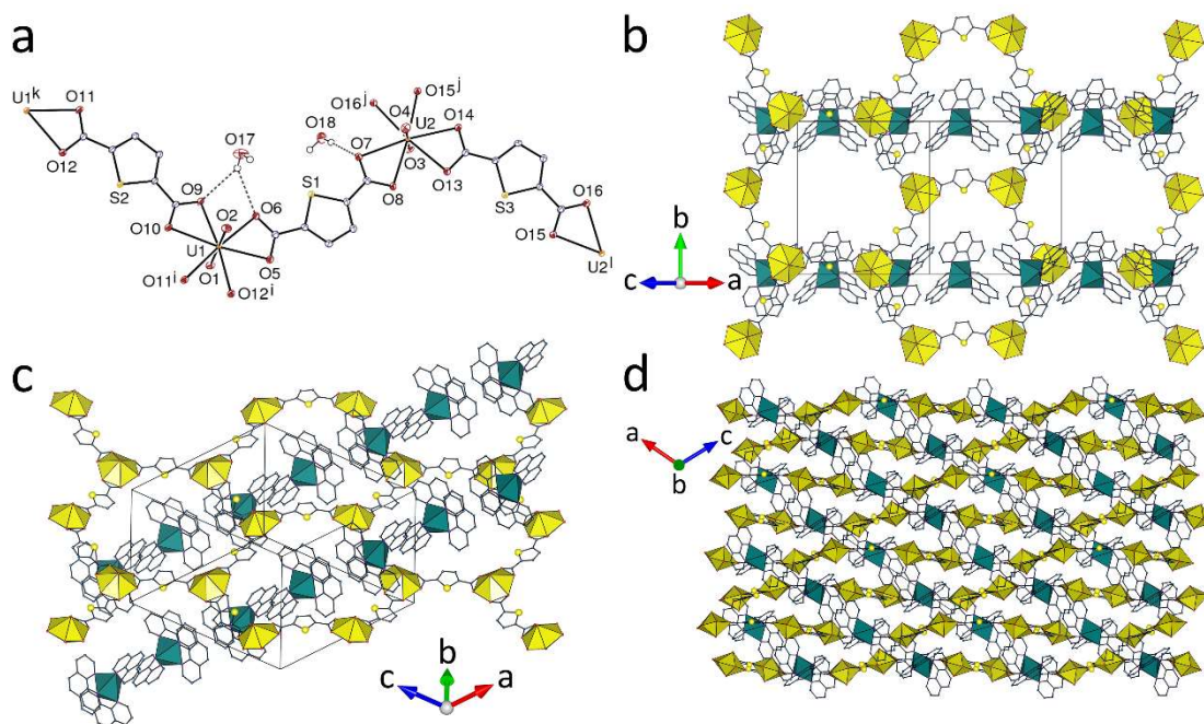
Figure 6. (a) View of compound 6 with displacement ellipsoids shown at the 50% probability level and hydrogen bonds shown as dashed lines. Symmetry codes: i = -x, y - 1/2, 3/2 - z ; j = 1 - x, y + 1/2, 1/2 - z ; k = -x, y + 1/2, 3/2 - z ; l = 1 - x, y - 1/2, 1/2 - z . (b and c) Two views of the diperiodic assembly with two inclined chains of counterions. (d) Packing with layers viewed edge-on and horizontal. Uranium coordination polyhedra are yellow and those of zinc green.
