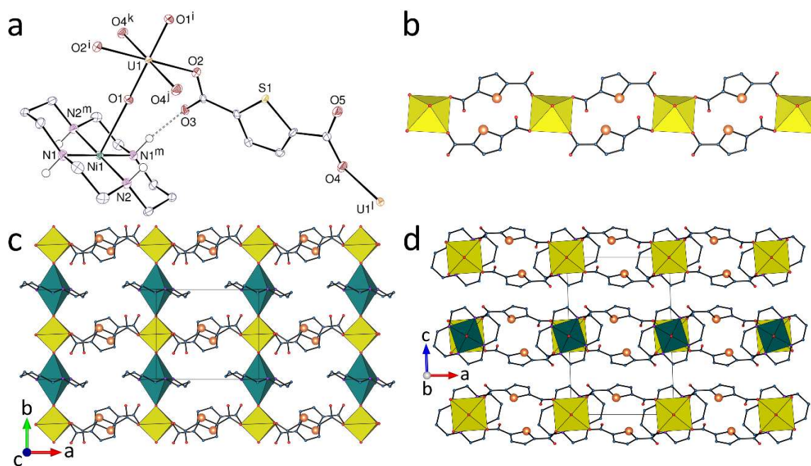
Figure 4. (a) View of compound 4 with displacement ellipsoids shown at the 50% probability level and the hydrogen bond shown as a dashed line. Symmetry codes: i = 2 - x, 1 - y, 1 - z ; j = 1 - x, 1 - y, 1 - z ; k = x + 1, y, z ; l = x - 1, y, z ; m = 2 - x, 2 - y, 1 - z . (b) The monoperiodic subunit. (c) The diperic assembly with coordination polyhedra yellow for uranium and green for nickel. (d) Packing with layers viewed edge-on.
