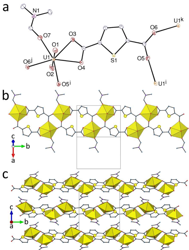
Figure 1. (a) View of complex 1 with displacement ellipsoids shown at the 50% probability level. Symmetry codes: i = 2 - x, 2 - y, 1 - z ; j = x, y - 1, z ; k = x, y + 1, z . (b) View of the monoperiodic assembly showing uranium coordination polyhedra. (c) View of the packing. Hydrogen atoms are omitted, and only one position of the disordered DMF molecule is shown in all views.
