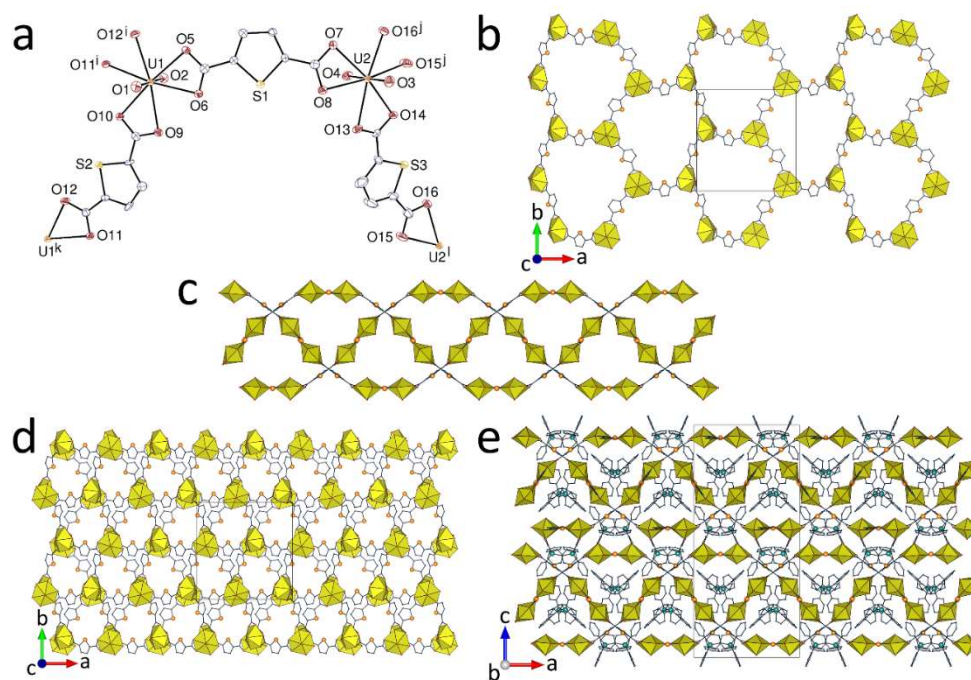
Figure 7. (a) View of compound 7 with displacement ellipsoids shown at the 50% probability level. Symmetry codes: i = 1 - x, y + 1/2, 3/2 - z ; j = 5/2 - x, y + 1/2, z ; k = 1 - x, y - 1/2, 3/2 - z ; l = 5/2 - x, y - 1/2, z . (b) The diperic assembly. (c and d) Two views of the threefold interpenetrating diperic networks. (e) Packing with layers viewed edge-on.
