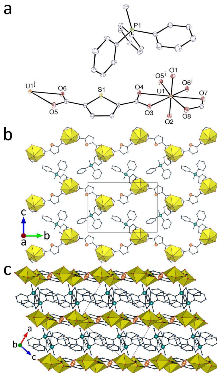
Figure 2. (a) View of compound 2 with displacement ellipsoids shown at the 50% probability level. Symmetry codes: Symmetry codes: i = 3/2 - x, y - 1/2, 3/2 - z ; j = 3/2 - x, y + 1/2, 3/2 - z . (b) Arrangement of chains in one layer with counterions. (c) Packing with layers viewed edge-on.
