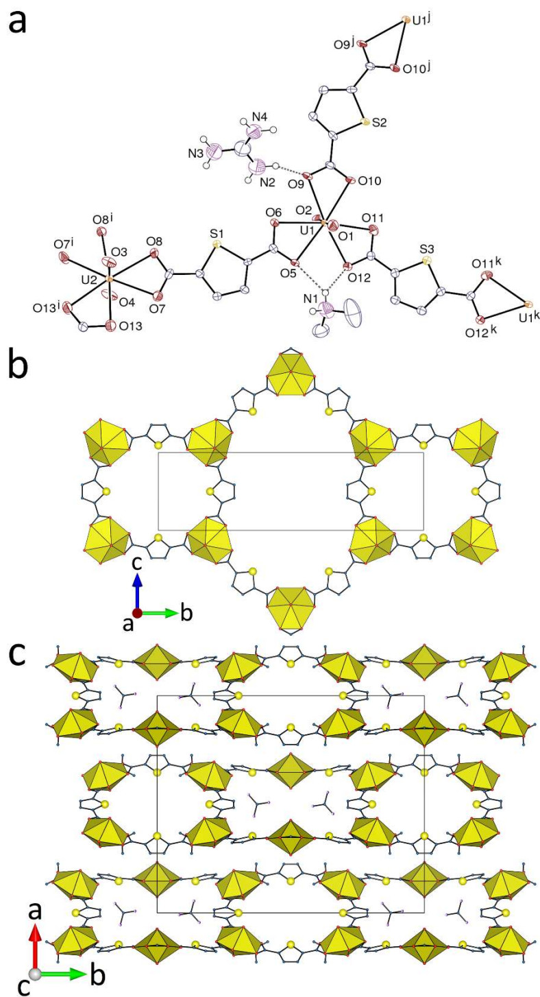
Figure 3. (a) View of compound 3 with displacement ellipsoids shown at the 50% probability level and hydrogen bonds shown as dashed lines. Only one position of the disordered counterion is represented. Symmetry codes: i = x, 1 - y, z ; j = 1 - x, y, -z - 1 ; k = x, 2 - y, z . (b) The monoperiodic assembly. (c) View of the packing.
