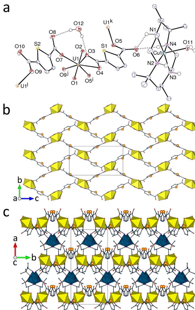
Figure 5. (a) View of compound 5 with displacement ellipsoids shown at the 50% probability level and hydrogen bonds shown as dashed lines. Symmetry codes: i = x, 1 - y, z - 1/2 ; j = x, 2 - y, z - 1/2 ; k = x, 1 - y, z + 1/2 ; l = x, 2 - y, z + 1/2 . (b) The dimeric assembly. (c) Packing with layers viewed edge-on. Uranium coordination polyhedra are yellow and those of copper blue.
