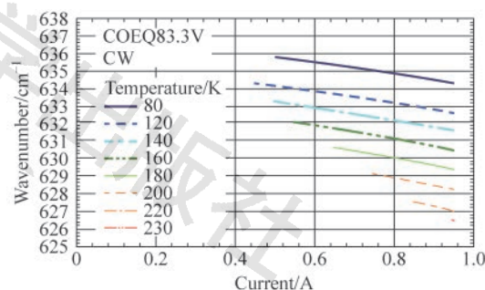
Figure 11: Example of current tunability at fixed temperature of our QCL ship
