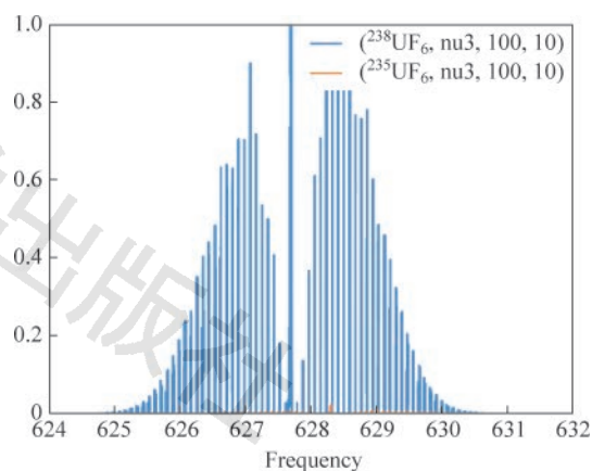
Figure 2: ^{235}\text{UF}_6 and ^{238}\text{UF}_6 cold bands at 10 K
