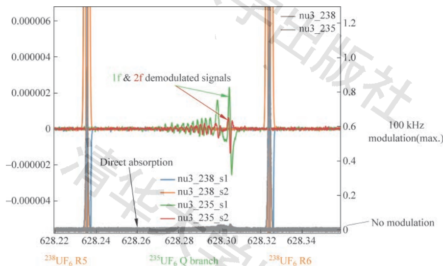
Figure 13: Simulation of noisy signals demodulated using the 2f/f scheme coming from the ^{235}\text{UF}_6 branch (red and green) to be compared to direct absorption (in grey)
