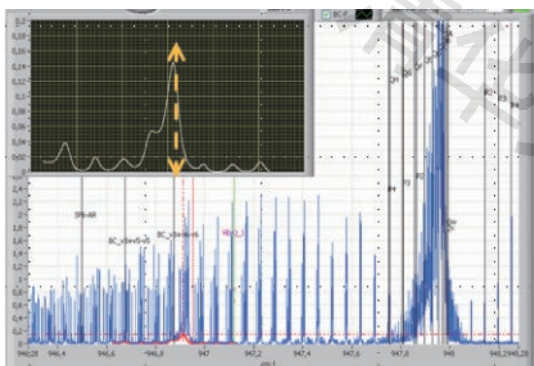
Figure 6: \nu_3 bands at 100 K vibrational temperature and at 20 K rotational temperature. hot bands (in red) are visible (for instance here involving \nu_5 bands vibration at 946.9 \text{ cm}^{-1} )
