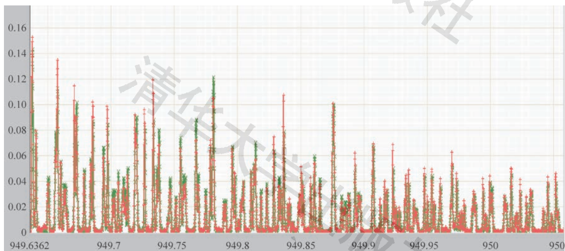
Figure 5: Theory and experiment agreement on the R side of the \nu_3 vibration of \text{SF}_6 , at 20 MHz resolution
