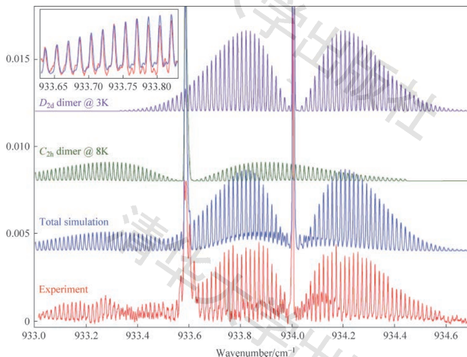
Figure 8: Parallel bands of the conformations # 1 and # 2 of the dimer (SF_6)_2 , summation compared to experimental spectrum
