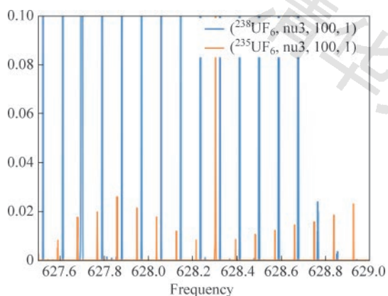
Figure 3: In orange, ^{235}\text{UF}_6 rotational lines are inside the rotational structure of ^{238}\text{UF}_6 , in blue
