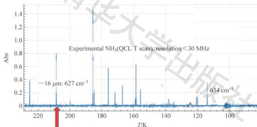
Figure 12: Experimental scan from 627 to 634 \text{cm}^{-1} with a 16 \mu\text{m} QC Laser. The red arrow indicates where the central position of the ^{235}\text{UF}_6 lines is on the ammonia spectrum
