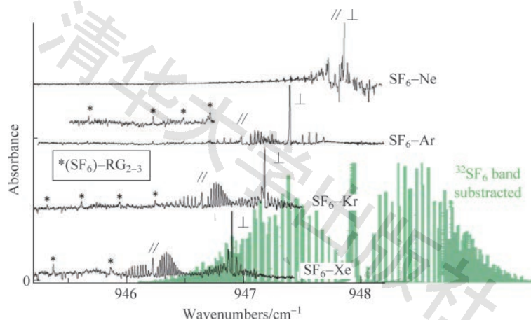
Figure 7: EC-QCL jet cooled pin hole spectra of both \nu_3 parallel bands of SF 6 -Rg heterodimers (Rg=Ne, Ar, Kr, Xe) with 0.12% SF 6 and 1% Rg diluted in 8 bar helium at an axial distance z=15 \text{ mm}
