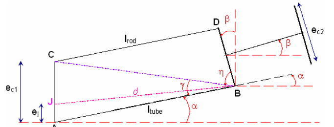
Fig. 17- Parallelogram distortion due to flexibilities
