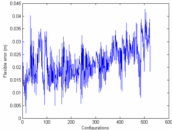
Fig. 19- distance (m) between the measured end effector's position and the calculated flexible position
