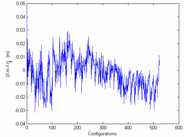
Fig. 12- Positioning error along the "z" axis
