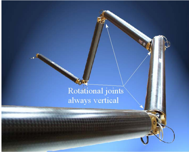
Fig. 1- PAC Robot Manipulator
