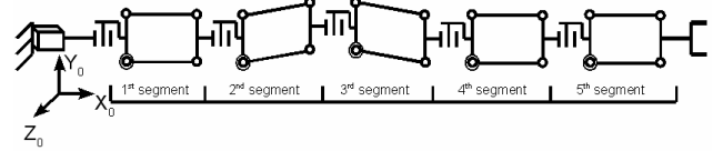
Fig. 3- PAC kinematics model with the parallelogram structure
