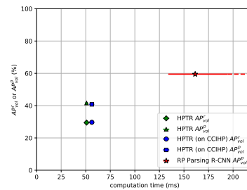
Fig. 4: Precision/time trade-off of HPTR on CIHP and CCIHP (on a TITAN X GPU), compared to RP Parsing R-CNN that achieved best precision and speed in multi-HP state of the art. HPTR is the fastest method and has constant time while RP Parsing R-CNN (a top-down approach) is more accurate but slower and not scalable: red horizontal solid line shows time variation with 2 to 18 people per image.
