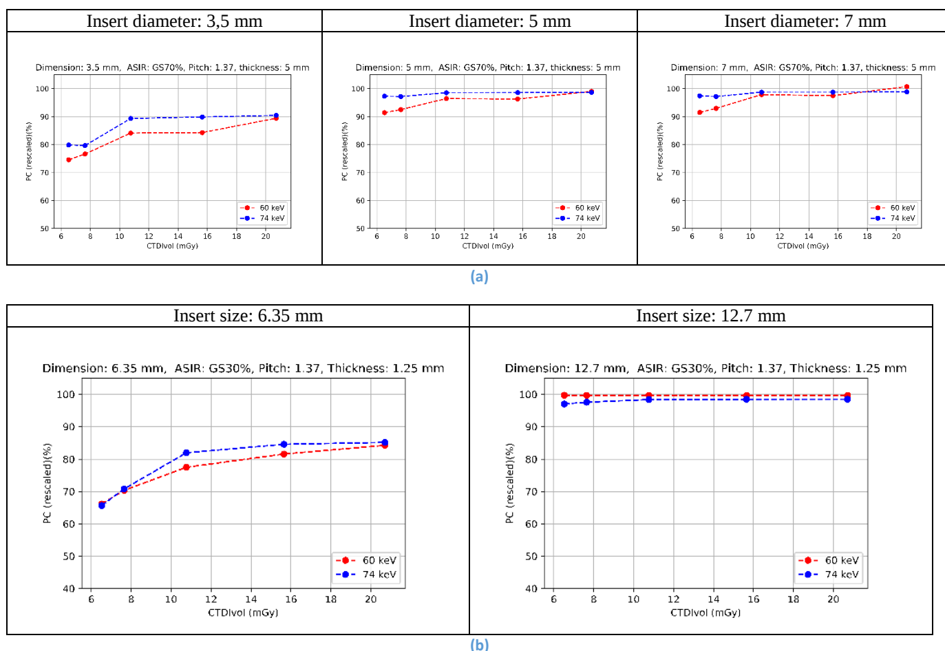
Figure 11: Percent correct (PC) calculated by the model observer after rescaling rNPWE_2 according to the CTDIvol, compared for GSI energy levels 60 keV and 74 keV. (a) Detection task, inserts of 3.5 mm, 5 mm and 7 mm diameter (epoxy resin), (b) discrimination task, inserts of 6.35 mm and 12.7 mm size (Teflon).
