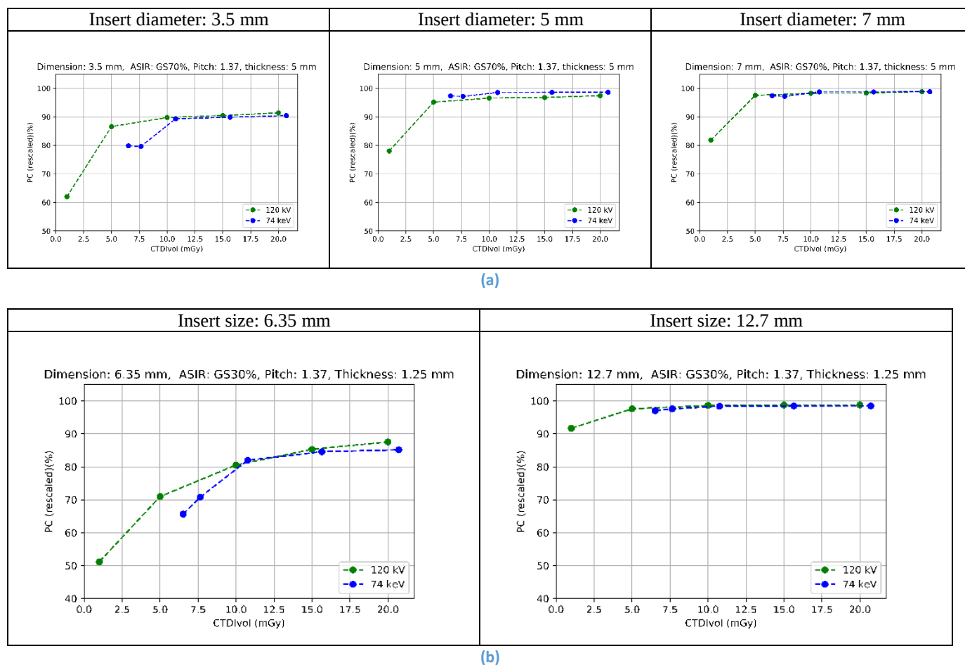
Figure 12: Comparison between the percent correct (PC) calculated by the model observer after rescaling rNPWE_2 according to the CTDIvol in both 120 kVp single-energy and 74 keV GSI energy level. (a) Detection task, inserts of 3.5 mm, 5 mm and 7 mm diameter (epoxy resin), (b) discrimination task, inserts of 6.35 mm and 12.7 mm size (Teflon).
