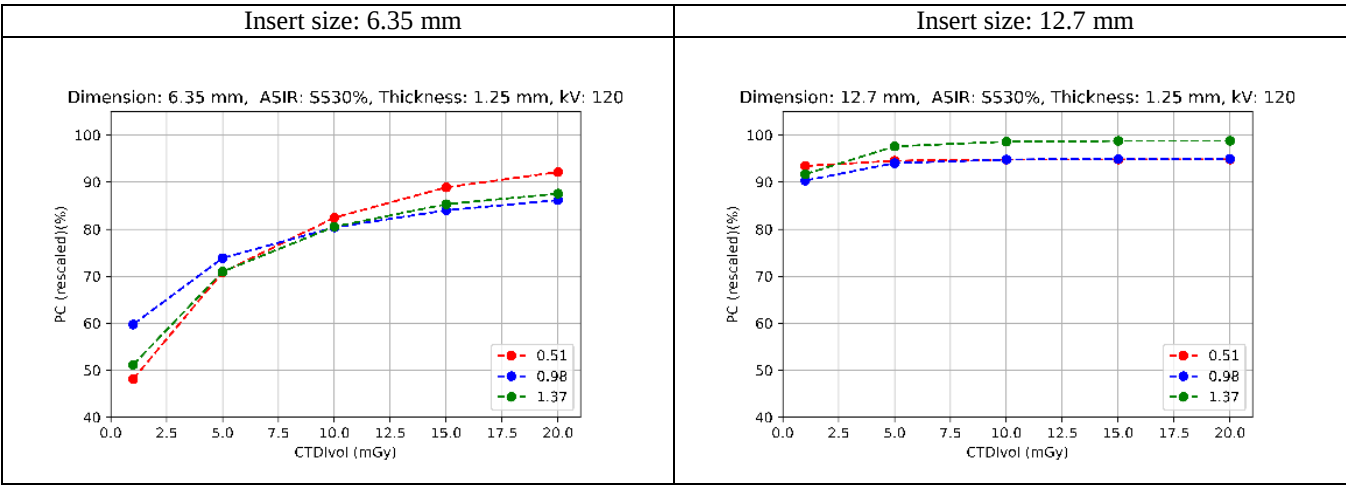
Figure 9: Comparison between the percent correct (PC) calculated by the model observer after rescaling rNPWE_2 according to the CTDIvol for the three values of pitch 0.516, 0.984 and 1.375. (a) Detection task, inserts of 3.5 mm, 5 mm and 7 mm diameter (epoxy resin), (b) discrimination task, inserts of 6.35 mm and 12.7 mm size (Teflon).
