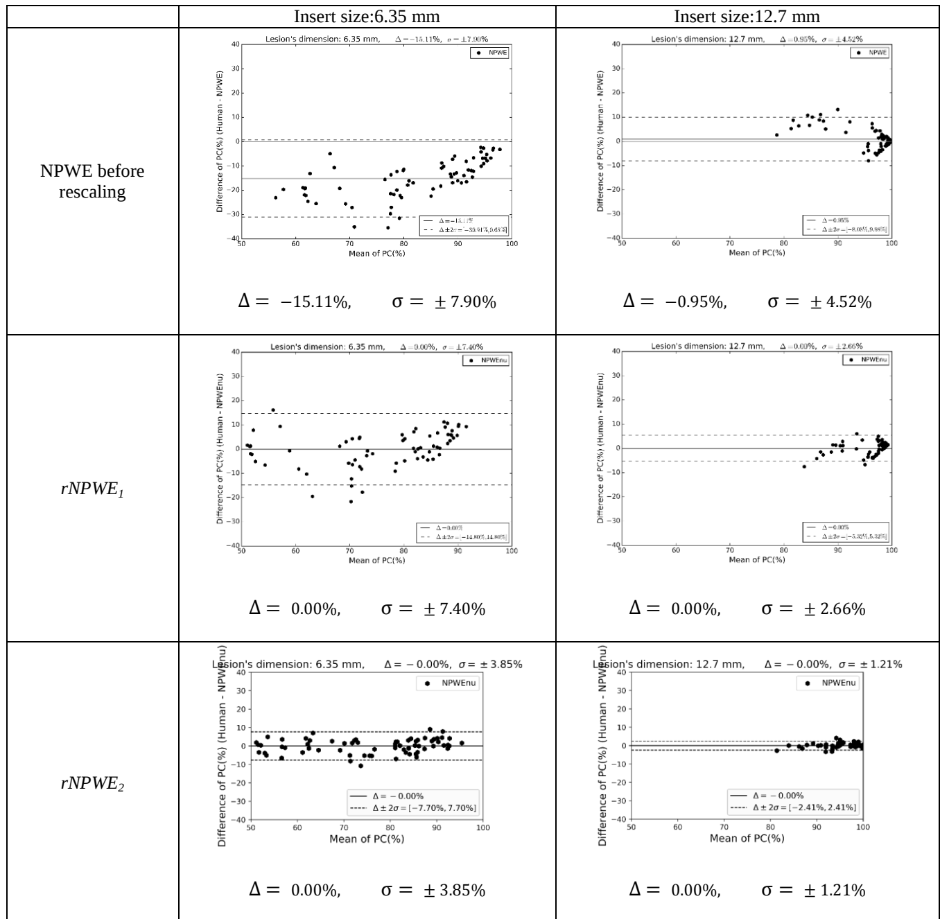
Figure 7: Bland-Altman plots corresponding to the NPWE model before rescaling and after rescaling using both cases. Means of differences \Delta and standard deviations of the differences \sigma are given for each case. (a) Detection task, inserts of 3.5 mm, 5 mm and 7 mm diameter (epoxy resin), (b) discrimination task, inserts of 6.35 mm and 12.7 mm size (Teflon).
