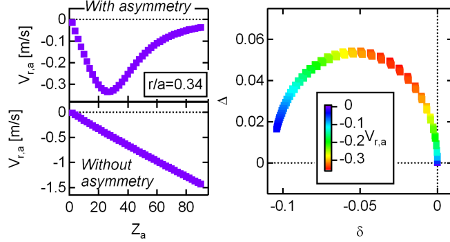
Figure 2: Radial flow with and without poloidal asymmetry, as a function of the impurity charge, and in the (\delta, \Delta) plane (right), for a peaked ion density.
