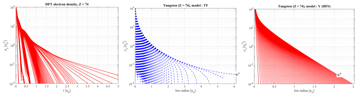
Fig. 1: Density of bound electrons averaged over solid angle for tungsten as a function of ion radius. Left: DFT model (code Gaussian, model PBE1PBE/gen/Auto (ANO-RCC) Integral= DKH2) [9], middle: TF model [10] and right: Y (HFS) model [12].
