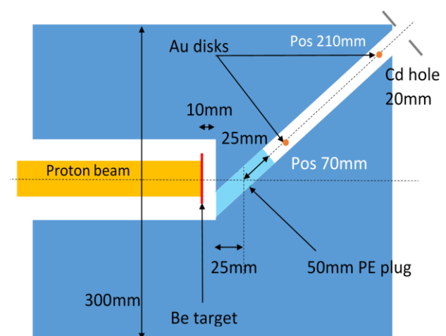
Fig. 2. Target and moderator assembly
