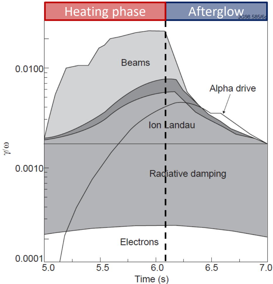
JET DT pulse 41723 – CASTOR-K, MISHKA [Sharapov NF 1999]
