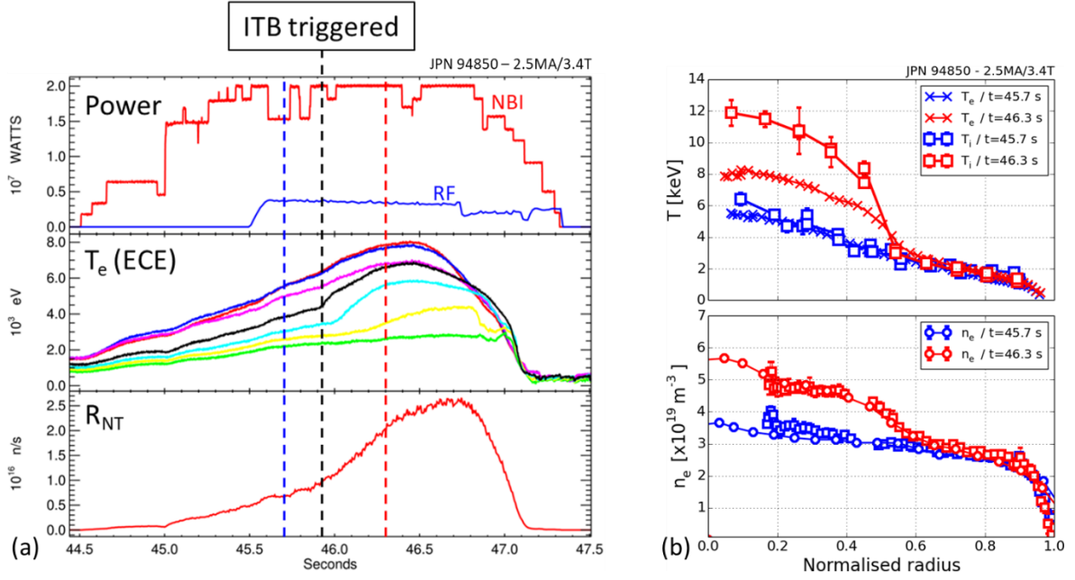
Figure 1: ITB triggered in JET pulse 94850. (a) From top to bottom: NBI and RF power; Electron temperature (ECE); neutron rate (b) Radial profiles (Top) Electron (x) and ion (squares) temperature profiles before ( t=45.7 s) and after ( t=46.3 s) the ITB triggering time ( t=45.9 s); (Bottom) Density profile.
