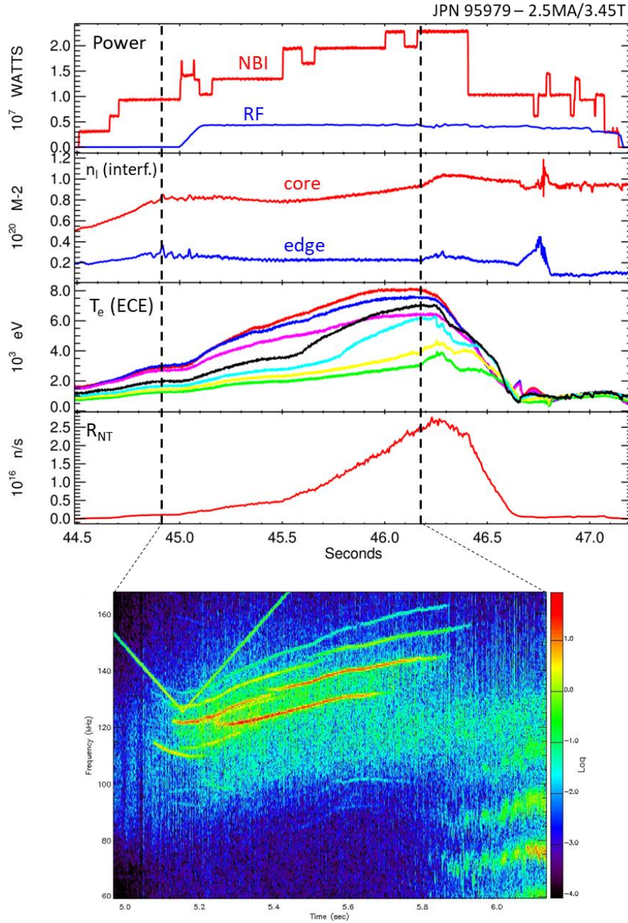
Figure 3 : JET pulse 95979. (Top) Time traces: NBI and RF power, core (channel 3) and edge (channel 4) line-integrated density (interferometry), electron temperature (ECE), DD neutron rate. (Bottom) Magnetic spectrogram. Core-localized TAEs excited by ICRH-driven ions with toroidal numbers 3-7 are observed in the presence of RF power, and disappear when the NBI power reaches its maximum.
