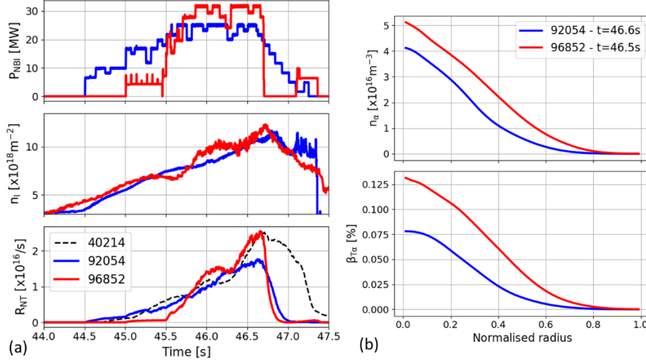
Figure 4: Comparison of JET pulses 92054 and 96852. (a) Time traces: NBI power, core line-integrated density (interferometry), DD neutron rate; also shown is the neutron rate for reference JET carbon wall pulse 40214, shifted by -0.31s. (b) TRANSP extrapolation to DT of pulses 92054 and 96852: (top) alpha density; (bottom) normalised alpha pressure.
