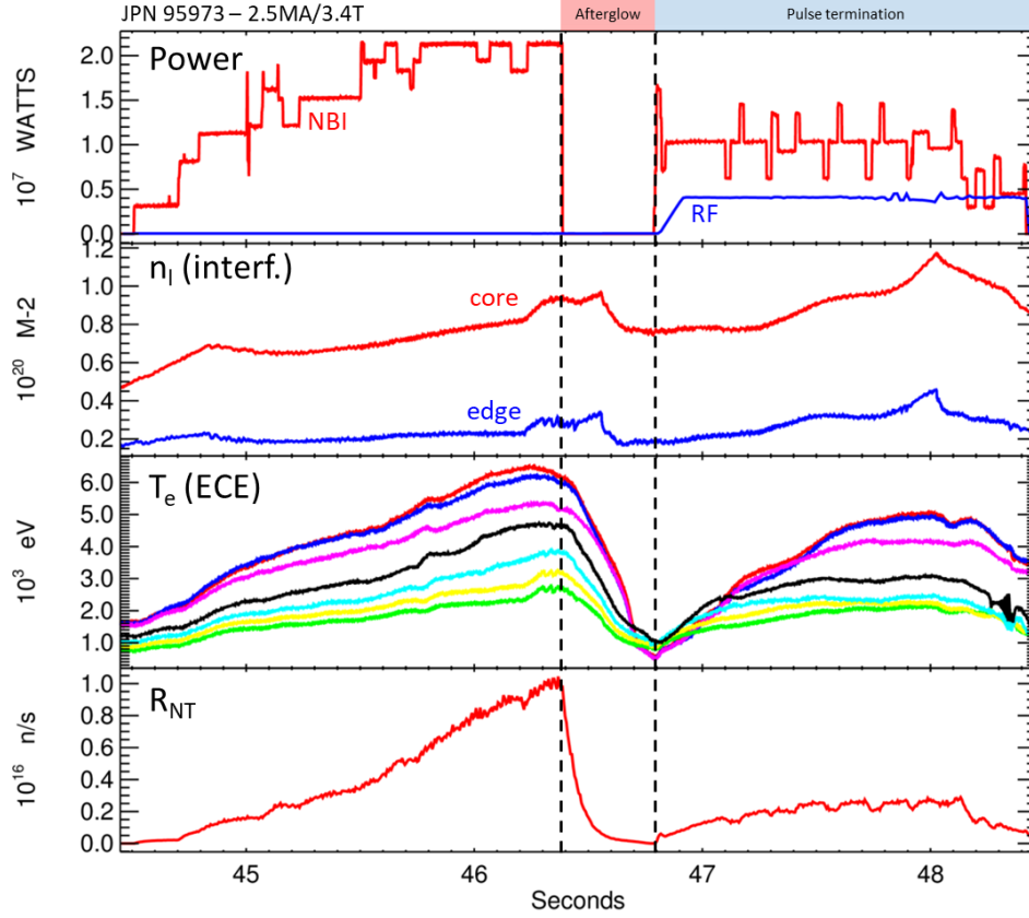
Figure 2 : Real-time triggering of afterglow phase in JET pulse 95973. From top to bottom: auxiliary power (NBI and RF); core (channel 3) and edge (channel 4) line-integrated density (interferometry), electron temperature (ECE), DD neutron rate.
