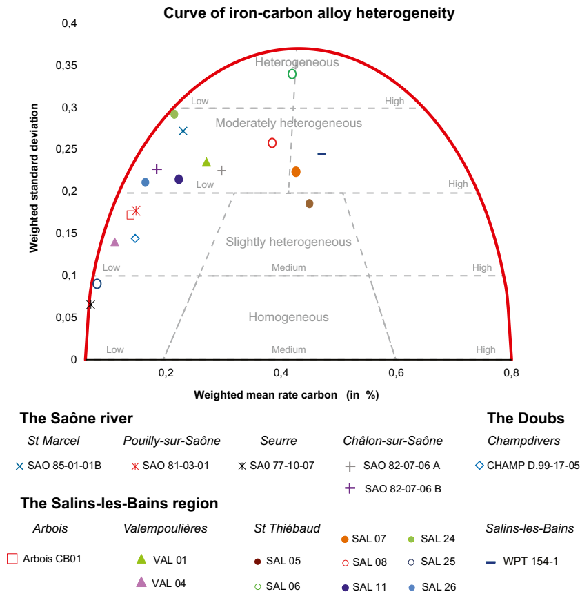
Figure 6 : Compositional domains of the iron-carbon alloy for the bars analysed (graphic from S. Bauvais-Leroy et al. 2017)
