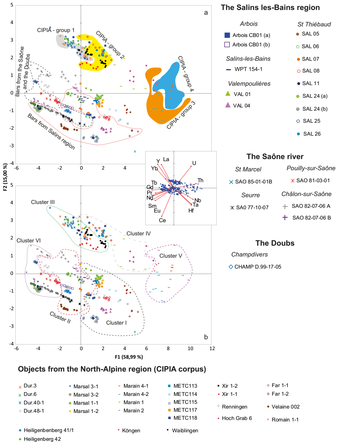
Figure 9 : PCA carried out on the xij of the currency-bars from the Saône River, the Doubs, the region of Salins-les-Bains and a comparative set of objects from the North-Alpine region (CIPIA corpus): a the provenance groups from the CIPIA study (Dillmann and al. 2017) and the geographical groups of the present study. b The clusters resulting from the AHC (refer to Fig. 8)
