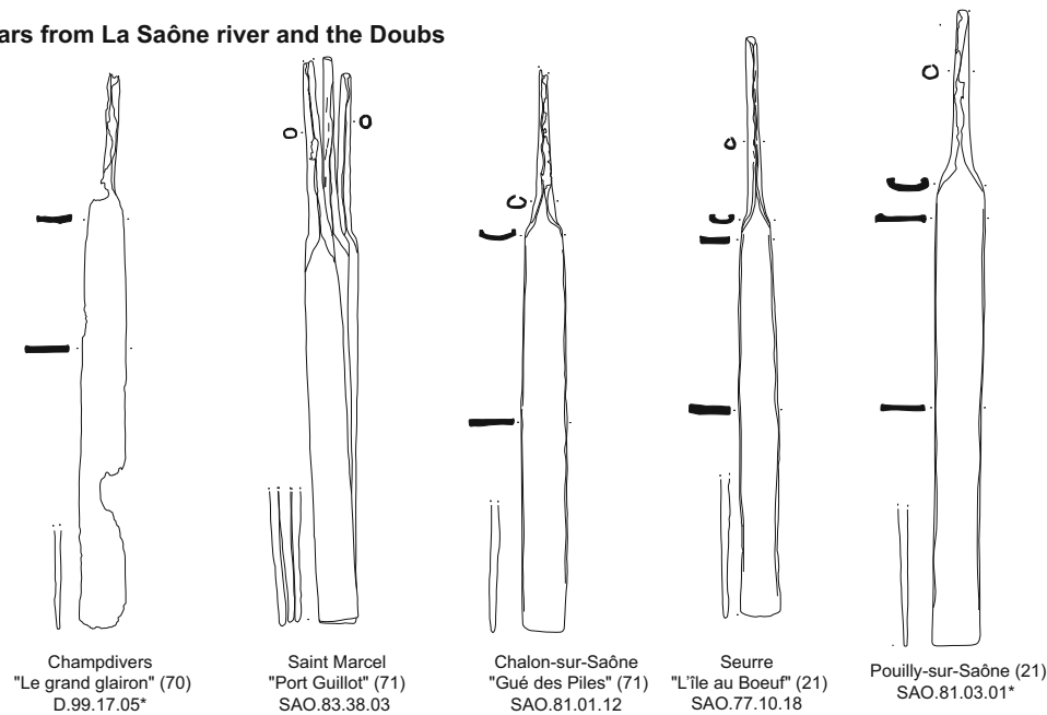
Figure 3 : The bars studied (a selection)
