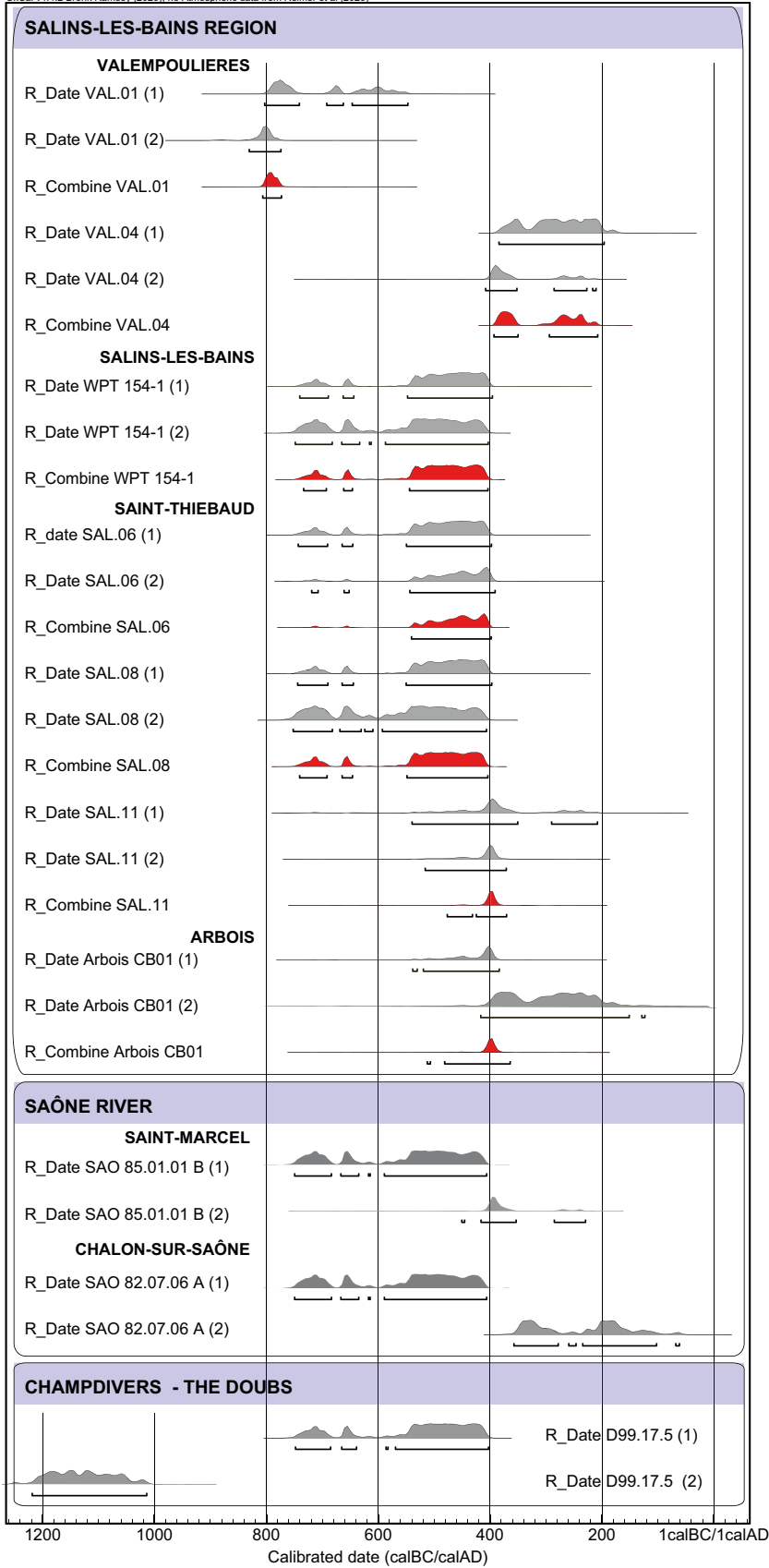
Figure 7 : Calibrated (95.4% probability ranges) and modelled radiocarbon dates (R-Combine) obtained for the currency-bars from the Saône River, the Doubs and the region of Salins-les-Bains. Calibration and modelling in OxCal v.4.4, IntCal2020
