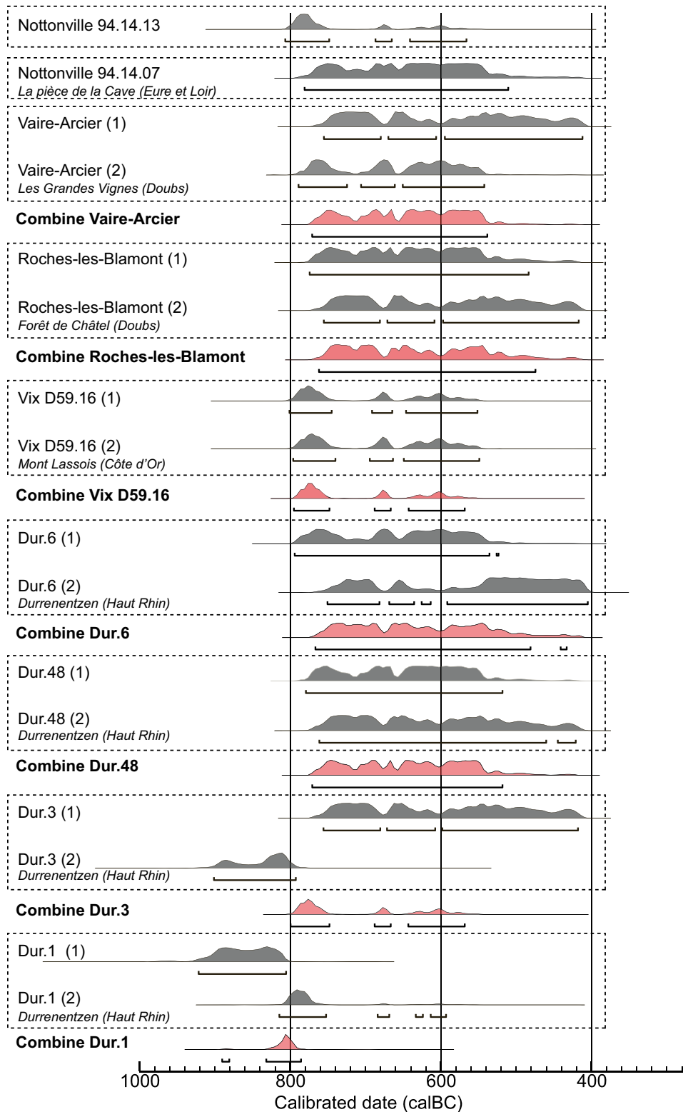
Figure 11 : Calibrated(95.4% probability ranges) and modelled radiocarbon dates (R-Combine) obtained for the bipyramidal semi-products. Calibration and modelling in OxCal v.4.4, IntCal2020
