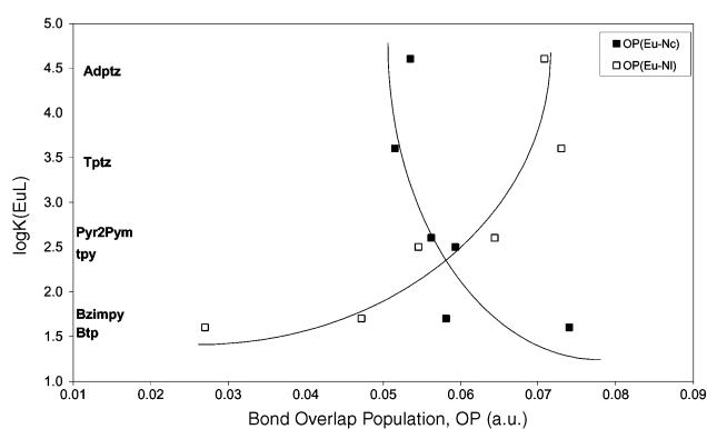
Fig. 4 Correlation between the Ln–N i and Ln–N c bond overlap populations in [EuL] 3+ complexes calculated in the gas phase and the stability constants of [EuLA 3 ] complexes (A = Cl - , ClO 4 - ) in MeOH–H 2 O solution (room temperature).
