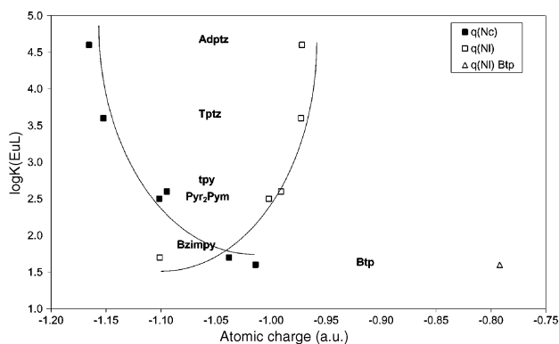
Fig. 3 Correlation between the atomic charges on N i and N c in [EuL] 3+ complexes calculated in the gas phase and the stability constants of [EuLA 3 ] complexes (A = Cl - , ClO 4 - ) in MeOH–H 2 O solution (room temperature).
