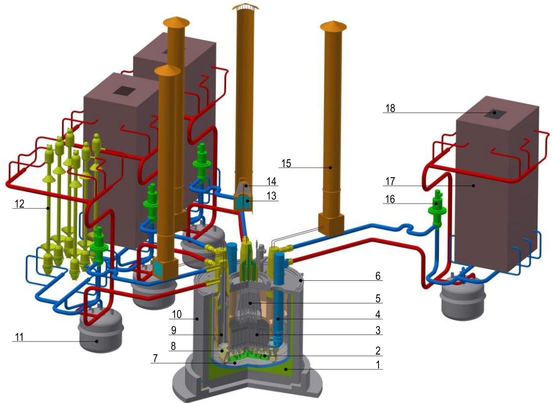
1: Insulation with steel liner 7: Main vessel 13: Window for air circulation (DHRS-1) 2: Core catcher 8: Strongback 14: Sodium-air HX (DHRS-1) 3: Core 9: IHX 15: Air chimney (DHRS-1) 4: Primary pump 10: Reactor pit 16: Secondary pump 5: Above-core structure 11: Secondary sodium tank 17: Casing of SGs (DHRS-2) 6: Pit cooling system (DHRS-3) 12: Steam generator 18: Window for air circulation (DHRS-2)
