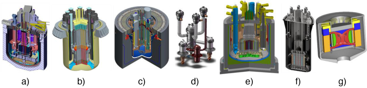
Fig. 1. Seven fast neutron systems supported by the considered EU project: ASTRID (a); ALFRED (b); MYRRHA (c); ALLEGRO (d); ESRF (e); SEALER (f); MSFR (g).
