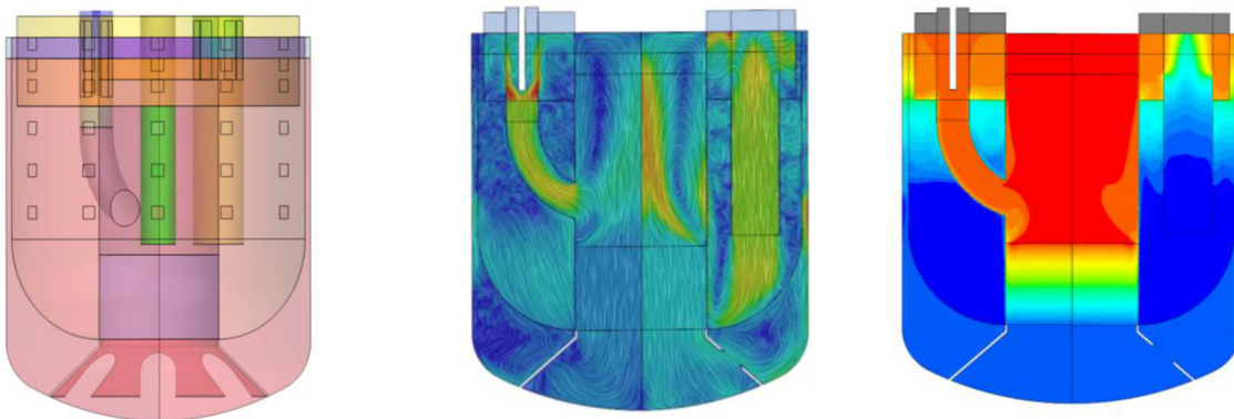
Fig. 9. CFD Model of ALFRED primary loop. (Courtesy of CRS4, SESAME Task 3.1.2).
