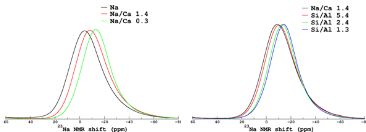
Figure 6: ^{23}\text{Na} NMR spectra for the glasses in series 1 and 3. The spectra for the glasses in series 2 are given in Supplementary Information.
