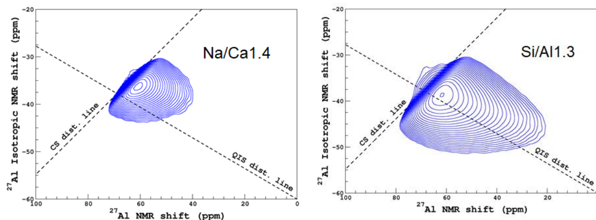
Figure 5: 2D ^{27}\text{Al} MQMAS NMR spectra for the Na/Ca 1.4 and Si/Al 1.3 glasses. Dashed lines represents the direction of spectral broadening induced by distribution of isotropic chemical shift (cs. dist. line) and quadrupolar interaction (second-order Quadrupolar Induced Shift – QIS - dist. line). These lines are helpful to determine the main contribution to the breadth of the MAS spectra.
