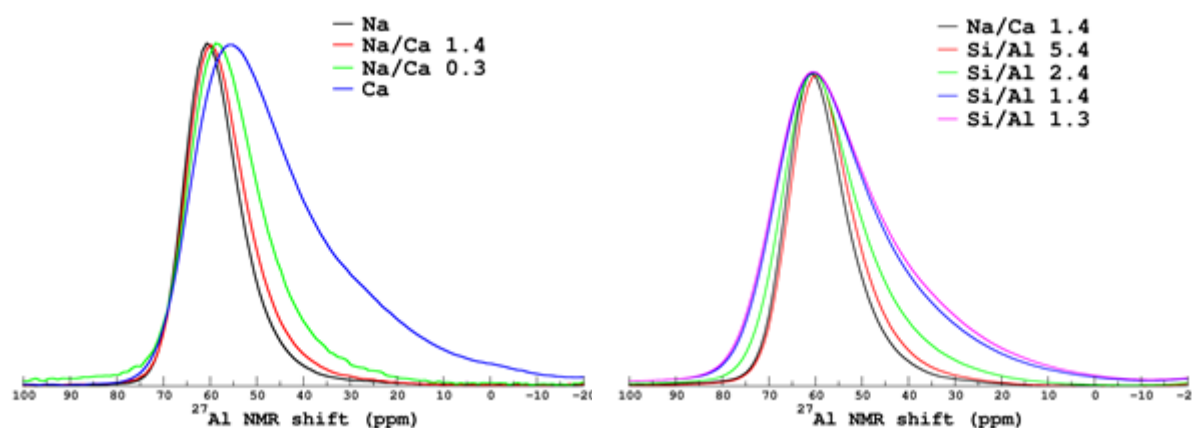
Figure 4: NMR spectra for ^{27}\text{Al} . Only glasses of series 1 and 3 are presented. The spectra for the glasses in series 2 are presented in the Supplementary Information.
