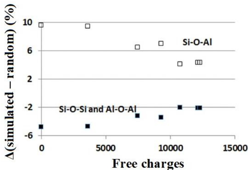
Figure 10: Difference between the percentages of Si-O-Si, Si-O-Al, and Al-O-Al measured by MD simulations and given by a random distribution model versus the quantity of free charges.
