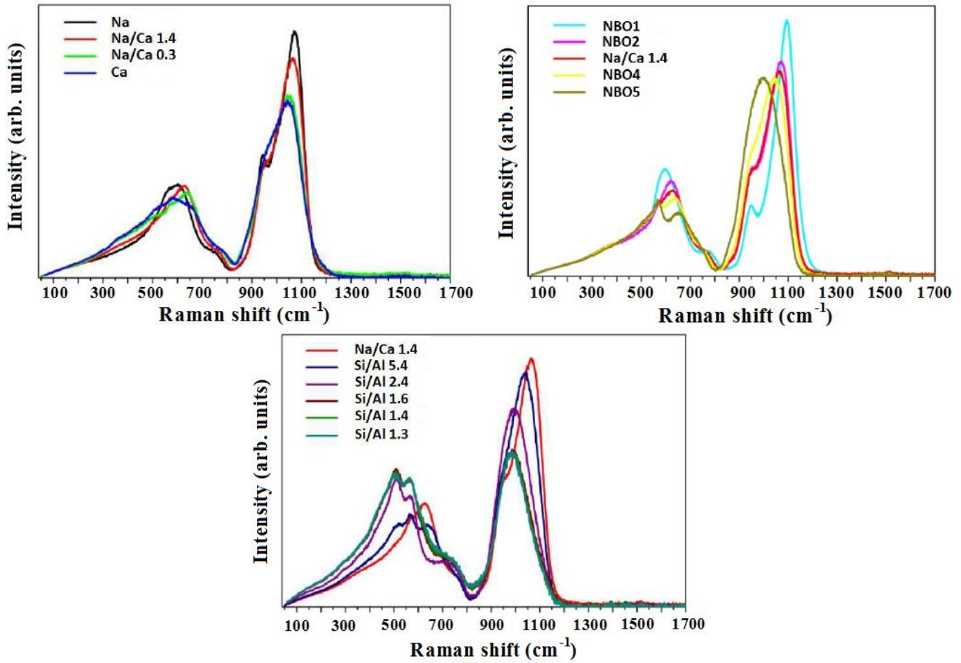
Figure 1: Raman spectra for the three series of glasses. The intensities have been normalized for the spectrum areas.
