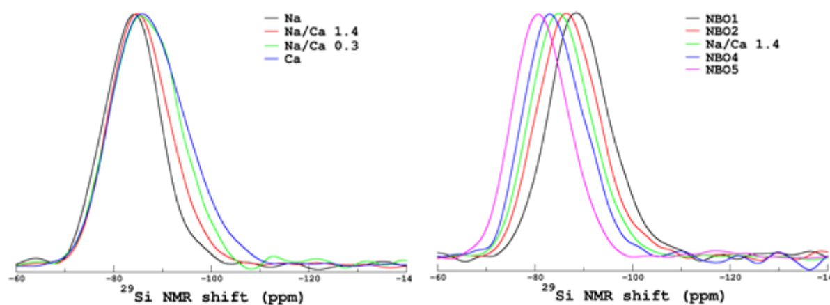
Figure 7: ^{29}\text{Si} NMR spectra for the glasses in series 1 and 2. The spectra for the glasses in series 3 are given in Supplementary Information.
