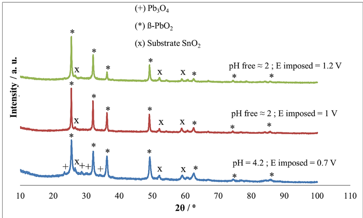
Figure 2: X-ray diffractograms of the adherent thin films obtained after the electrochemical treatment of a lead solution ( [\text{Pb(II)}] = 27 \text{ mg}\cdot\text{L}^{-1} ), for different values of imposed potentials and pH (pH free \approx 2 and pH adjusted to 4.2 by adding of \text{NaOH} (1M)), at room temperature, with stirring of the solution (250 rpm) for 24 hours. S ( \text{SnO}_2 ) = 3 \text{ cm}^2
