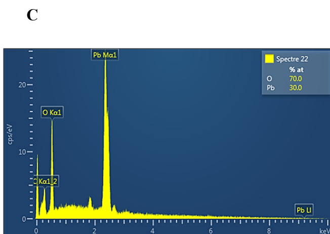
Figure 3: SEM observations and analyzes by EDS of the adherent thin films obtained after the electrochemical treatment of a lead solution ( [Pb(II)] = 27 \text{ mg. L}^{-1} ), at room temperature, with stirring, for 24 hours, with different values of imposed potential and pH, S (\text{SnO}_2) = 3 \text{ cm}^2 . (A) \text{pH} = 4.2 , E = 0.7 \text{ V} ; (B) free \text{pH} \approx 2 , E = 1 \text{ V} ; (C) free \text{pH} \approx 2 , E = 1.2 \text{ V} . Scale (x3000: 0.3 \text{ cm} = 2 \mu\text{m} ) and (x 20000: 0.6 \text{ cm} = 1 \mu\text{m} ).
