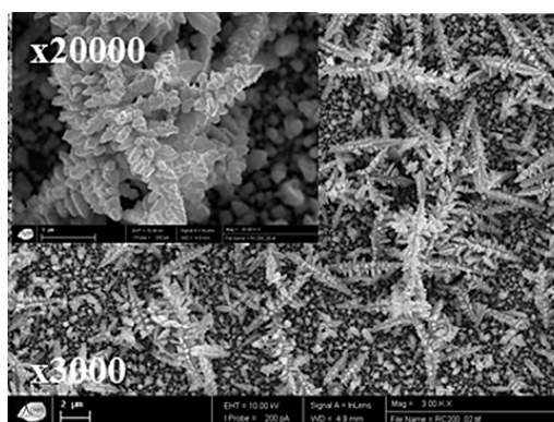
Figure 3: SEM observations and analyzes by EDS of the adherent thin films obtained after the electrochemical treatment of a lead solution ( [Pb(II)] = 27 \text{ mg. L}^{-1} ), at room temperature, with stirring, for 24 hours, with different values of imposed potential and pH, S (\text{SnO}_2) = 3 \text{ cm}^2 . (A) \text{pH} = 4.2 , E = 0.7 \text{ V} ; (B) free \text{pH} \approx 2 , E = 1 \text{ V} ; (C) free \text{pH} \approx 2 , E = 1.2 \text{ V} . Scale (x3000: 0.3 \text{ cm} = 2 \mu\text{m} ) and (x 20000: 0.6 \text{ cm} = 1 \mu\text{m} ).
