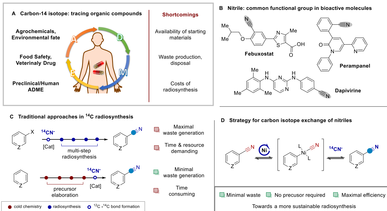
Fig. 1. Development of nitrile carbon isotope exchange. (A) societal field impacted by routine ^{14}\text{C} -radiosynthesis of organic compounds. (B) representative examples of bioactive molecules bearing nitrile moieties. (C) Multi-steps approaches commonly utilized to insert ^{14}\text{C} -nitriles into biologically relevant molecules. (D) Nitrile carbon isotope exchange. The blue colored circles denote the positions of the labeled carbon atoms.
