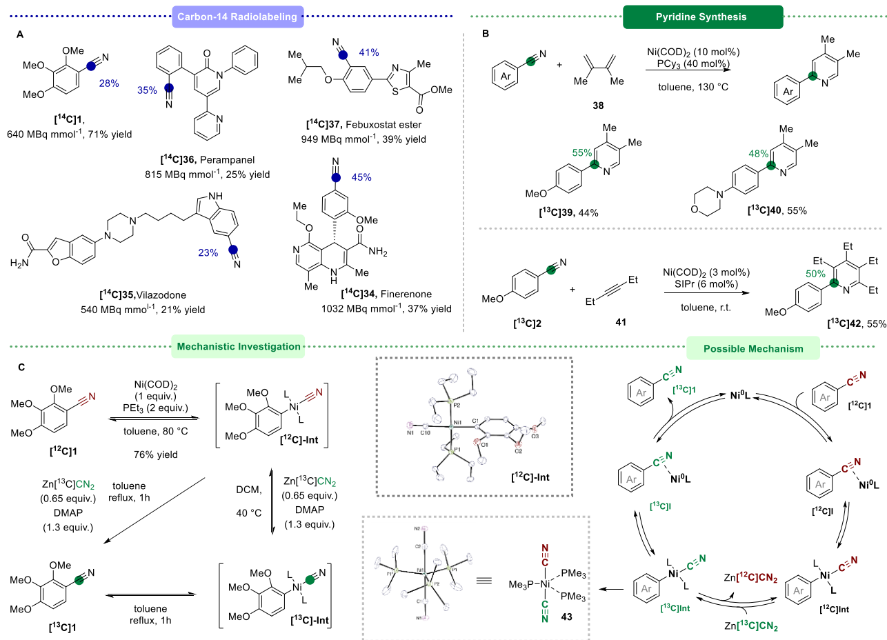
Fig. 3: (A) Ni-catalyzed carbon-14 labeling. (B) Synthesis of labeled pyridine by [4+2]cycloaddition reactions. (C) Mechanistic investigation on the nitrile isotope exchange and preliminary mechanistic proposal.
