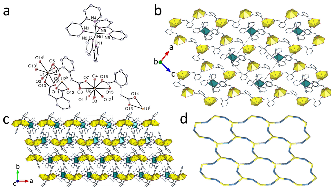
Figure 3. (a) View of complex 3 with displacement ellipsoids drawn at the 50% probability level. Solvent molecules and hydrogen atoms are omitted. Symmetry codes: i = x + 1, y, z + 1 ; j = x - 1, y, z ; k = x + 1, y, z ; l = x - 1, y, z - 1 . (b) View of the diperiodic coordination polymer and the counterions with uranium coordination polyhedra yellow and those of nickel green. (c) Packing with layers viewed edge-on. (d) Nodal representation of the network (yellow, uranium nodes; blue, dicarboxylate links; same orientation as in (b)).
