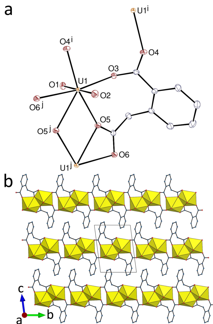
Figure 1. (a) View of complex 1 . Displacement ellipsoids are drawn at the 50% probability level. Symmetry codes: i = 2 - x, 2 - y, 1 - z ; j = 1 - x, 1 - y, 1 - z . (b) View of the packing with uranium coordination polyhedra colored yellow. Hydrogen atoms are omitted in both views.
