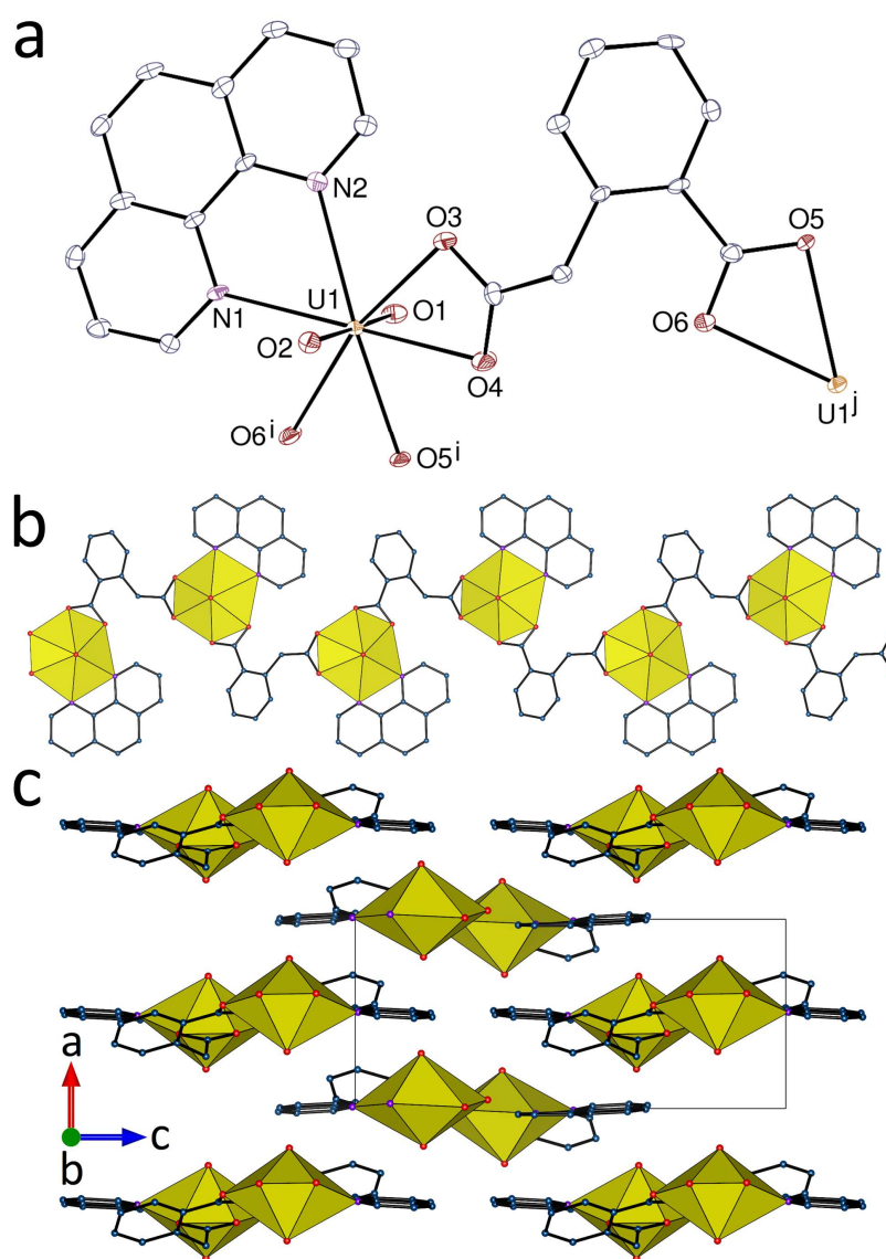
Figure 2. (a) View of complex 2 . Displacement ellipsoids are drawn at the 50% probability level. Symmetry codes: i = 1 - x, y - 1/2, 3/2 - z ; j = 1 - x, y + 1/2, 3/2 - z . (b) View of the monoperiodic coordination polymer. (c) View of the packing. Hydrogen atoms are omitted in all views.
