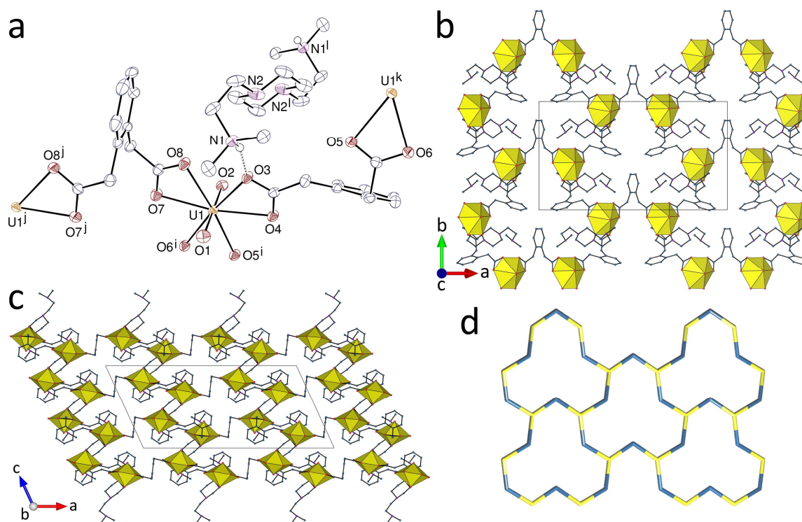
Figure 5. (a) View of complex 5 with displacement ellipsoids drawn at the 50% probability level. Solvent molecules and carbon-bound hydrogen atoms are omitted, and the hydrogen bond is shown as a dashed line. Symmetry codes: i = 3/2 - x, y + 1/2, 3/2 - z ; j = 2 - x, y, 3/2 - z ; k = 3/2 - x, y - 1/2, 3/2 - z ; l = 3/2 - x, 1/2 - y, 1 - z . (b) View of the dimeric coordination polymer with the counterions. (c) Packing with layers viewed edge-on. (d) Nodal representation of the network (yellow, uranium nodes; dark blue, dicarboxylate links; same orientation as in (b)).
