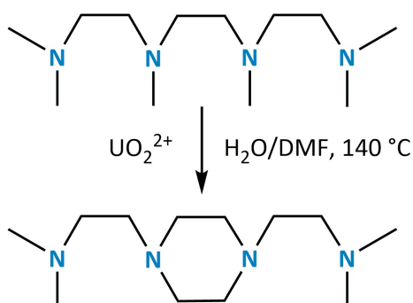
Scheme 1. Transalkylation of Me 6 trien during the synthesis of complex 5 . Protonation of the amine groups is not indicated.
