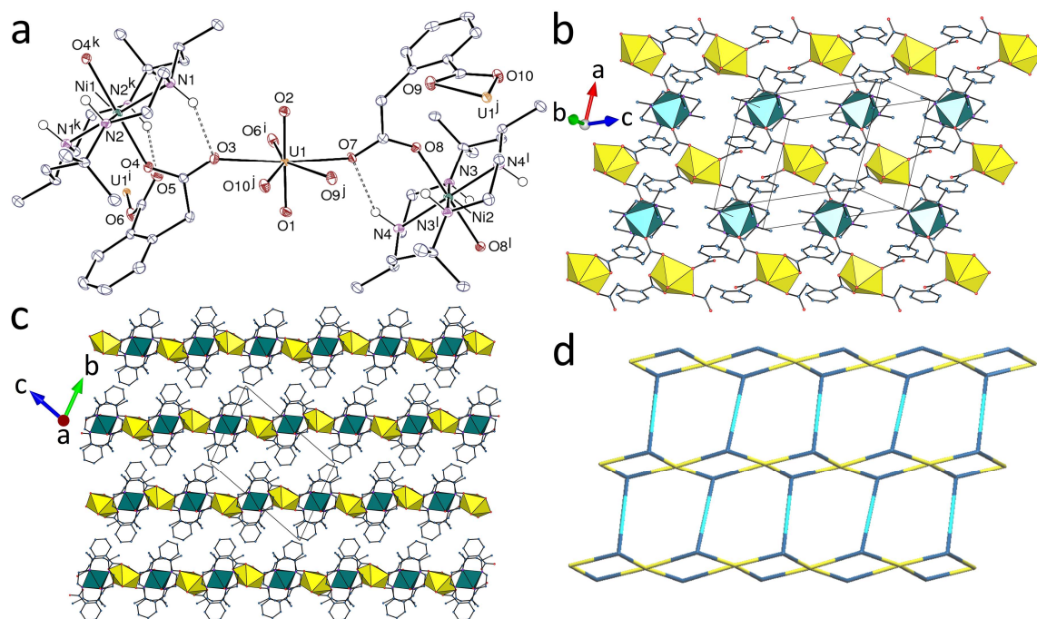
Figure 4. (a) View of complex 4 with displacement ellipsoids drawn at the 50% probability level. Carbon-bound hydrogen atoms are omitted and hydrogen bonds are shown as dashed lines. Symmetry codes: i = 1 - x, 1 - y, -z ; j = 1 - x, -y, 1 - z ; k = 2 - x, 1 - y, -z ; l = -x, -y, 1 - z . (b) View of the diperiodic coordination polymer with uranium coordination polyhedra yellow and those of nickel green. (c) Packing with layers viewed edge-on. (d) Nodal representation of the network (yellow, uranium nodes; dark blue, dicarboxylate nodes; light blue, nickel links; orientation slightly rotated with respect to that in (b)).
