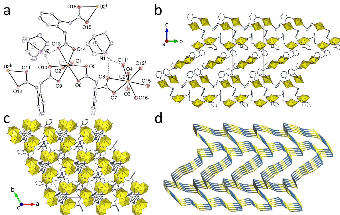
Figure 6. (a) View of complex 6 with displacement ellipsoids drawn at the 50% probability level. Solvent molecules and carbon-bound hydrogen atoms are omitted, and the hydrogen bonds are shown as dashed lines. Symmetry codes: i = 1 - y, x - y, z + 1/3 ; j = 1 - y, x - y + 1, z + 1/3 ; k = y - x + 1, 1 - x, z - 1/3 ; l = y - x, 1 - x, z - 1/3 . (b) and (c) Two views of the triperiodic framework with hydrogen atoms, counterions and solvent molecules omitted. (d) Nodal representation of the framework (yellow, uranium nodes; dark blue, dicarboxylate links; orientation slightly rotated with respect to that in (b)).
