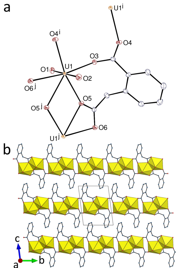
Figure 1. (a) View of complex 1. Displacement ellipsoids are drawn at the 50% probability level. Symmetry codes: i = 2 - x, 2 - y, 1 - z ; j = 1 - x, 1 - y, 1 - z . (b) View of the packing with uranium coordination polyhedra colored yellow. Hydrogen atoms are omitted in both views.
