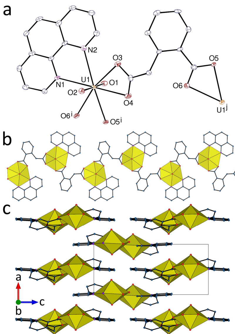
Figure 2. (a) View of complex 2 . Displacement ellipsoids are drawn at the 50% probability level. Symmetry codes: i = 1 - x, y - 1/2, 3/2 - z ; j = 1 - x, y + 1/2, 3/2 - z . (b) View of the monoprotic coordination polymer. (c) View of the packing. Hydrogen atoms are omitted in all views.
