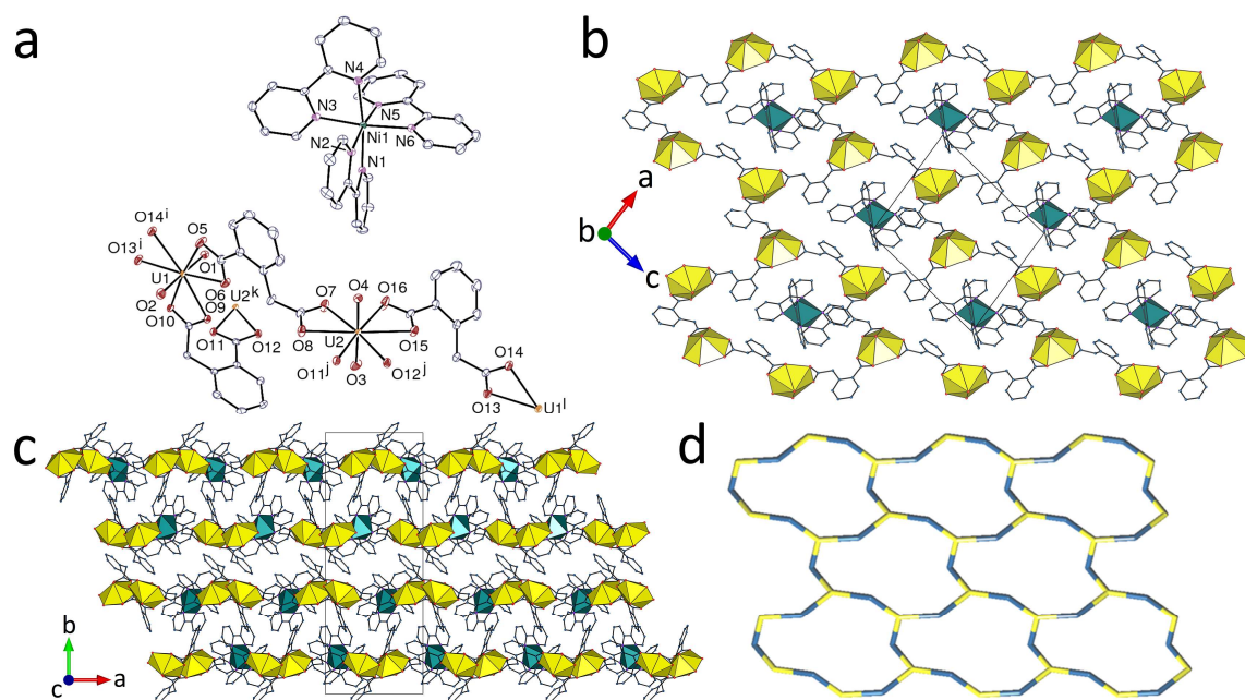
Figure 3. (a) View of complex 3 with displacement ellipsoids drawn at the 50% probability level. Solvent molecules and hydrogen atoms are omitted. Symmetry codes: i = x + 1, y, z + 1 ; j = x - 1, y, z ; k = x + 1, y, z ; l = x - 1, y, z - 1 . (b) View of the diperiodic coordination polymer and the counterions with uranium coordination polyhedra yellow and those of nickel green. (c) Packing with layers viewed edge-on. (d) Nodal representation of the network (yellow, uranium nodes; blue, dicarboxylate links; same orientation as in (b)).
