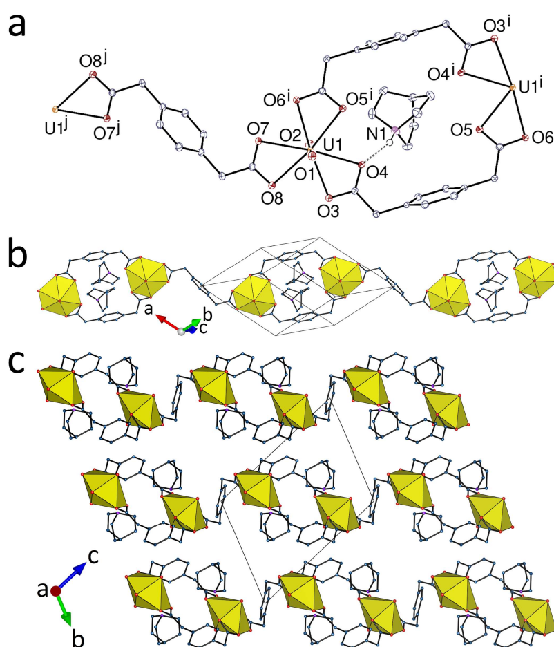
Figure 7. (a) View of complex 7 with displacement ellipsoids drawn at the 50% probability level. Solvent molecules and carbon-bound hydrogen atoms are omitted, and the hydrogen bond is shown as a dashed line. Symmetry codes: i = 1 - x, 1 - y, 1 - z ; j = -x, 2 - y, 2 - z . (b) View of the monoperiodic coordination polymer with the counterions. (c) Packing with chains viewed obliquely.
