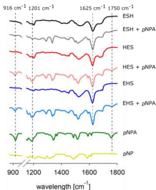
Figure 3. ATR-FTIR transmittance spectra of lyophilized solutions, of peptides ( 250\text{ }\mu\text{M} ) and their equimolar mixtures with p NPA. Spectra of p NPA and p NP are provided for comparison.
