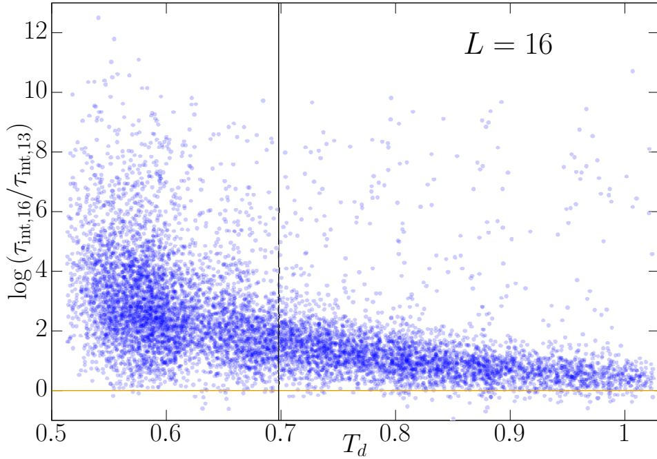
Figure 6. Scatter plot of \log(\tau_{\text{int},16}/\tau_{\text{int},13}) versus T_d . The lattice size is L = 16 , \tau_{\text{int},16} is the relaxation time for N_T = 16 ( T_{\text{min}} = 0.479 ), \tau_{\text{int},13} is the relaxation time for N_T = 13 ( T_{\text{min}} = 0.698 ), T_d is the temperature of chaos from a dynamical point of view (defined in the variational method) of the simulation with N_T = 16 . Same disorder samples in the two simulations. The vertical black line represents the minimum temperature simulated in the N_T = 13 simulation. (We added a small Gaussian white noise to T_d , which is a discrete variable, to avoid the cluttering of data in vertical lines).
