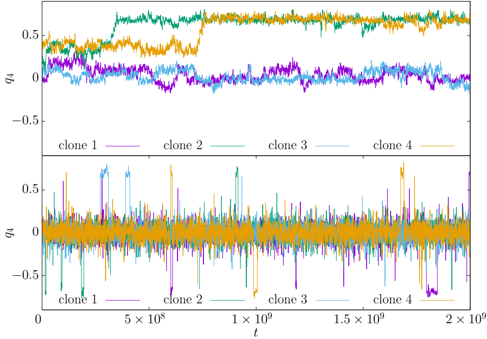
Figure E1. Top: Monte Carlo history for the overlap q_4(t) , see Eq. (E.12), as computed for each of the four clones in the truncated simulation (see text). Note that our simulation time is much too short to expose the symmetry q_4 \leftrightarrow -q_4 . As a consequence, we know for sure that thermal equilibrium has not been reached for the truncated simulation. Bottom: As in top panel, for the first four clones in one of our standard simulations with N_T = 24 temperatures (there were 10, completely independent, standard simulations). For each clone, the overlap q_4(t) changes sign many times along the simulation (as it is to be expected for a well equilibrated simulation). Note that, with small probability, each clone reaches a state where |q_4| \sim 0.8 . These events, which are not observed for the other three overlaps q_a a = 1, 2, 3 , make particularly interesting to study the dynamics of q_4 .
