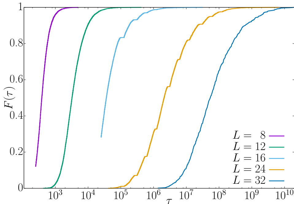
Figure 3. Empirical probability distribution of \tau for L = 8, 12, 16, 24 and 32 . For L = 8 and L = 12 some of the samples have \tau smaller than our minimal resolution (if \tau < n_{\text{Met}} we cannot compute it safely). We show only the part of the distribution function that can be safely computed.
