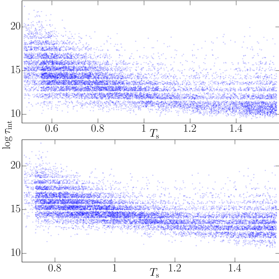
Figure 10. Scatter plot of \log(\tau_{\text{int}}) against T_s . We show L = 16 (top) and L = 24 (bottom). T_s is the temperature where X_{T_{\min}, T}^J presents the maximum (negative) slope.
