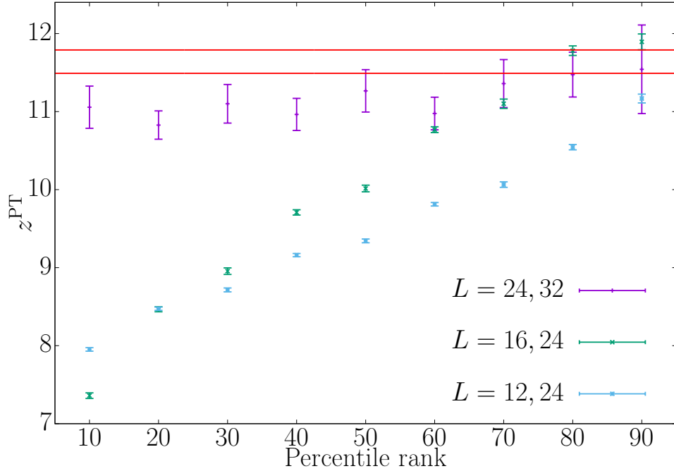
Figure 4. The effective exponent z^{\text{PT}}(L_1, L_2, p) for three different pairs of lattice sizes (12,24), (16,24) and (24,32) as a function of the percentile rank p . The two horizontal lines are the bounds for the off-equilibrium value z = 11.64(15) (see Eq. (19)). The numerical values of z^{\text{PT}} for the largest pair are compatible with the off-equilibrium value.
