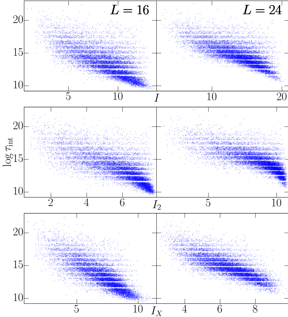
Figure 9. Scatter plot of \log(\tau_{\text{int,var}}) versus the integrated chaotic parameter I . We present data for two lattice sizes and for the three definitions of the integrated chaotic parameter defined in the text ( I , I_2 and I_X ). The pattern of depleted horizontal bands is due to our choice of a few l_{\text{blo}} .
