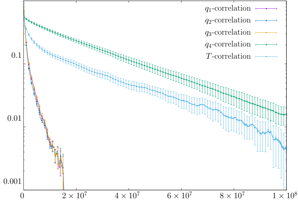
Figure E2. Equilibrium time dependent correlation functions, as computed from the standard simulation with N_T = 24 . We consider five observables, one related to temperature (computed from the piece-wise linear function with T^* = T_3 , see Table 1 and Sect. 4.1), and the overlaps q_a with a = 1, 2, 3, 4 defined in Eq. (E.12). The fact that the T and q_4 correlations become parallel in this semi-logarithmic scale indicates that we are safely computing the exponential auto-correlation time (which is independent of the observable). Instead, the q_{a=1,2,3} correlations do not become parallel to the other curves, at least not within the range we can measure, which probably indicates that the amplitudes A_{n=1, q_{a=1,2,3}} , see Eq. (E.10), are much smaller for these observables.
