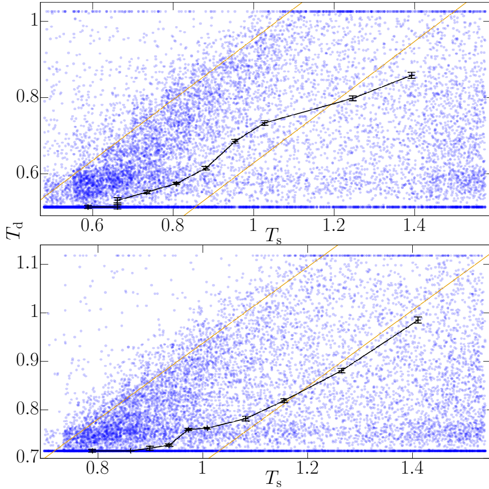
Figure D1. Scatter plot of T_d versus T_s . We present the L = 16 -data (top) and the L = 24 -ones (bottom). Points are calculated with an special procedure. First, samples are classified on deciles according to \log(\tau_{\text{int}}) . The points coordinates were obtained by computing the median T_d and the median T_s within each decile (errors from bootstrap). The red parallel lines enclose the area of over-density that presents a higher correlation for later recount.
