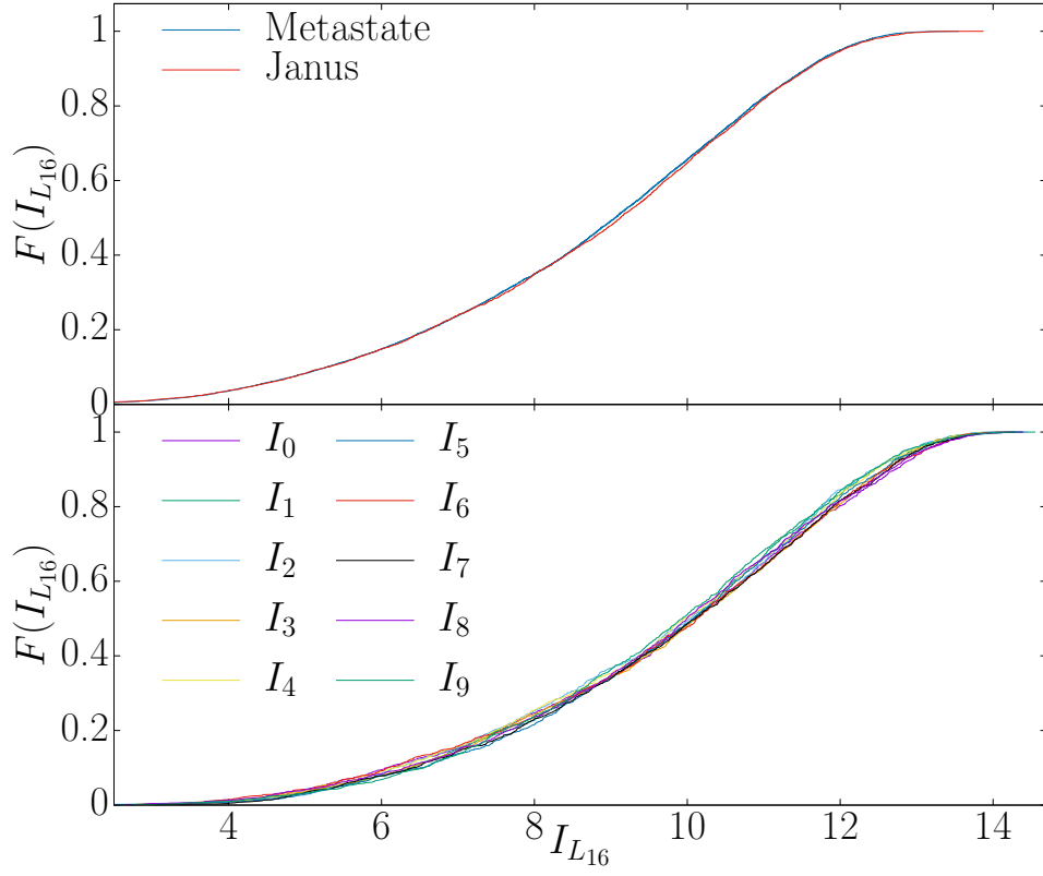
Figure B2. Empirical probability distribution function of the integrated chaotic parameter. Top We compare the distribution (labeled as "Metastate") obtained with our particular choice of samples with the distribution obtained from 4000 fully independent samples (data from Janus). Bottom: Distributions obtained for the 10 inner samples plotted separately. Averaging over the metastate (over the outer couplings) reduces strongly the fluctuations between the inner samples.
