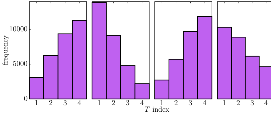
Figure E3. For each of the four clones in the truncated simulation, we indicate the histogram of temperature (i.e. the number of times that \pi_t(\alpha) = 1 , or \pi_t(\alpha) = 2 , etc.). The temperature state was sampled every 5 \times 10^4 Metropolis sweeps (per clone). Had the simulation equilibrated, we would have expected the occupation histograms to be uniform.
