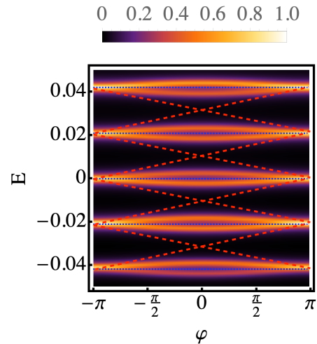
Figure 7. LDOS averaged over 6 sites x \in [90, 95] , plotted as a function of the phase difference \varphi on the horizontal axis and energy on the vertical axis. We set L = 200 , V_A = 3.5 and \mu = 1.5 . The perfect Andreev limit is denoted by the red dashed lines while the particle-in-the-box by the blue dotted lines.
