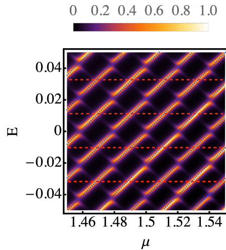
Figure 6. LDOS averaged over 6 sites x \in [90, 95] , plotted as a function of the chemical potential on the horizontal axis and energy on the vertical axis. We set L = 200 , V_A = 3.5 and \mu varies between 1.46 and 1.54, so that \alpha \approx 1 does not vary with \mu . The phase difference is set to \varphi = 0 . The perfect Andreev limit is denoted by the red dashed lines while the particle-in-the-box by the blue dotted lines.
