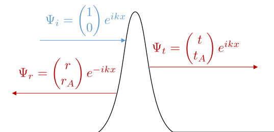
Figure 3. Schematics of an “Andreev” impurity with the incoming, reflected and transmitted plane waves.
