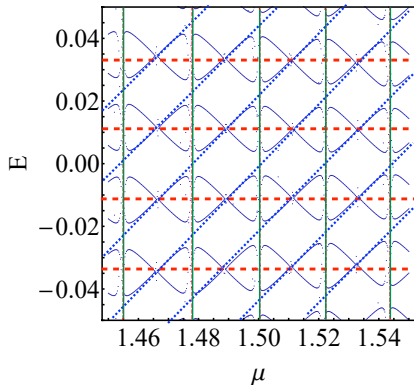
Figure 10. Energies of the ABS within the continuum model plotted as a function of the chemical potential. The vertical green lines mark the values of the chemical potential at which the analytical perturbative approach becomes invalid due to singularities in Eq. (29). Here, exactly as in Fig. 6, we have set V_A = 3.5 , \varphi = 0 and L = 200 . Additionally, we have fixed m = 0.5 . The perfect Andreev limit is denoted by the red dashed lines while the particle-in-the-box by the blue dotted lines.
