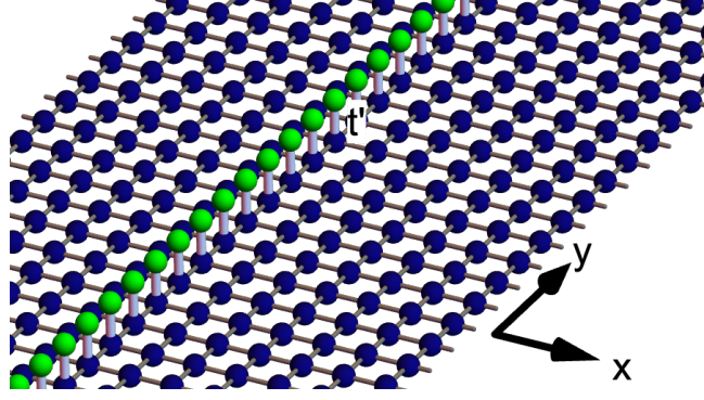
Figure S1. A schematic of the magnetic impurity sites (green atoms) above the superconducting surface (dark blue atoms).
