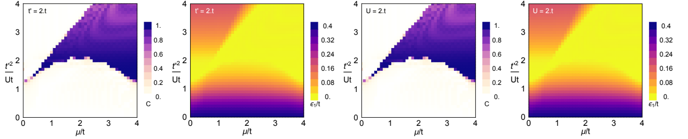
Figure S2. A comparison of the lowest energy state energy \epsilon_1 and its Majorana polarization C for the impurities defined as sites above the two-dimensional lattice. Here we take \lambda = 0.2t , and \Delta = 0.4t . Either t' or U are kept constant and the other term is varied, as labelled in the figures.
