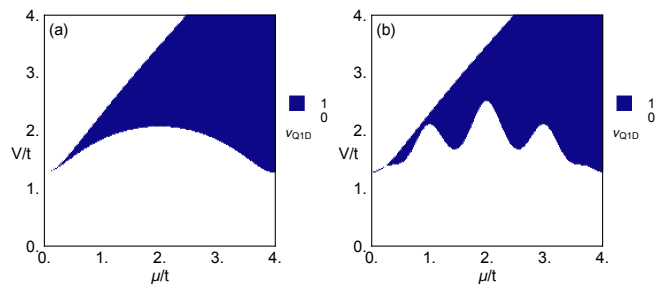
Figure 3. The quasi-one-dimensional invariant, \nu_{\text{Q1D}} , for (a) N_x = 51 and (b) N_x = 11 .
