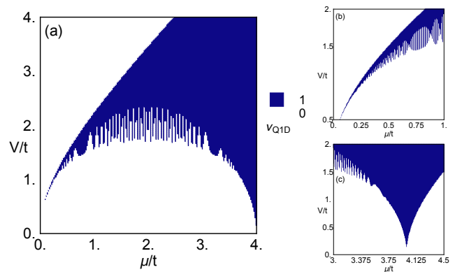
Figure 4. The quasi-one-dimensional invariant for \lambda = \Delta = 0.005t for N_x = 1001 . Small panels (b,c) demonstrate the parts of the phase diagram close to \mu/t = 0 and \mu/t = 4 in a higher resolution.
