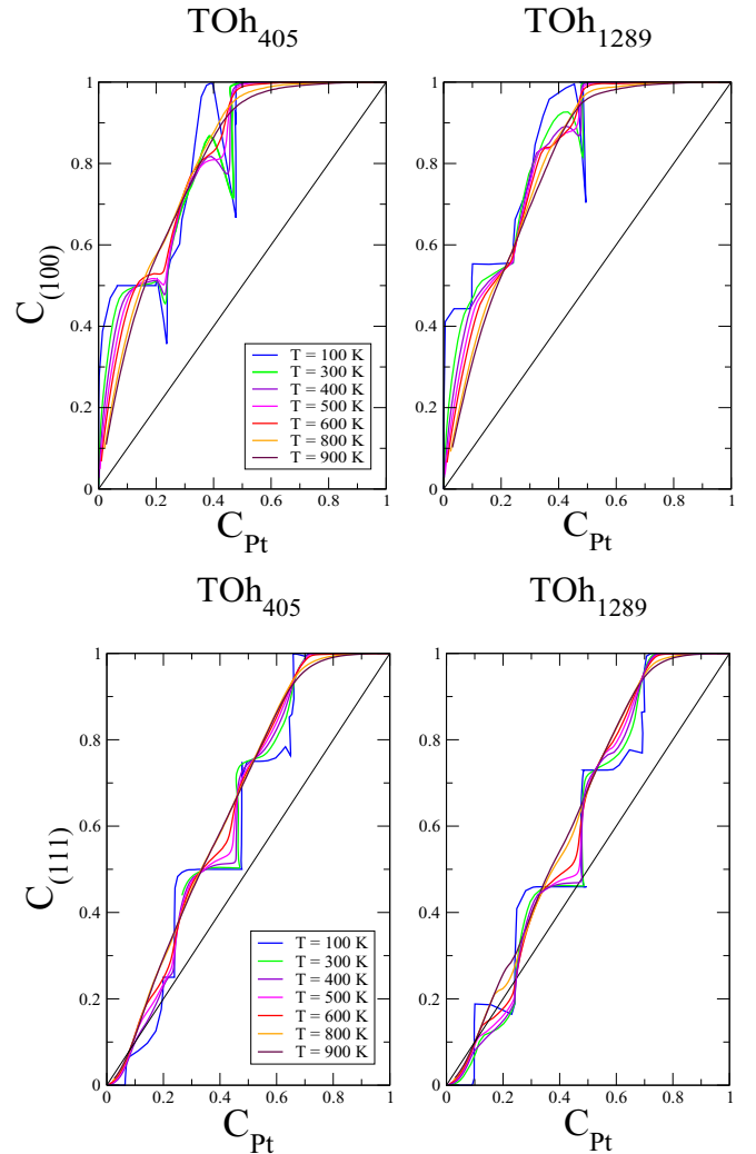
FIG. 11. (Color online) Segregation isotherms at various temperatures from 100 to 900 K for the (100) and the (111) facets of the clusters of 405 and 1289 atoms as a function of the cluster core Pt concentration.
