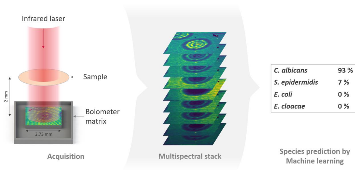
Figure 1. Mid-infrared multispectral lensless imaging principle.
