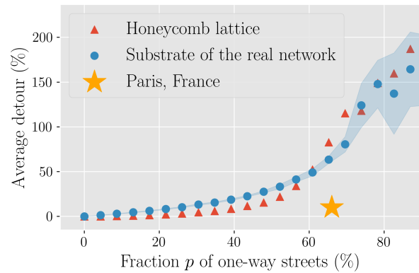
FIG. 5: Average detour \bar{\eta} as a function of the fraction p of randomly chosen one-way streets in the city of Paris (France). In this statistical process, the detour increases with the fraction p . We note, however, that the empirical detour in the real world (indicated by a star symbol) remains below the result expected from a random uniform distribution of one-way streets. This indicates that the actual choice of one-way streets in Paris is far from what would be obtained by a random choice of one-way streets and favors small detours. We compare these results to the obtained for a honeycomb lattice, whose degree distribution is close the Paris.
