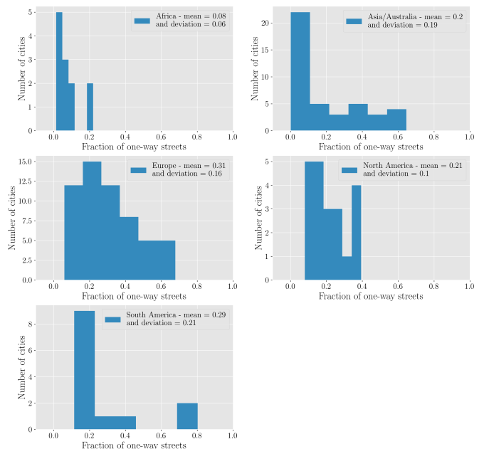
FIG. 1: Distribution of the fraction p of one-way streets for the five continents (the fraction is defined as the total length of one-way streets over the total length of the network).
