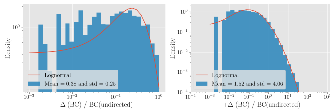
FIG. 3: Distribution of the relative variation \Delta of the betweenness centrality (BC) due to one-way streets in the Parisian network for negative (the BC decreases) and positive values of \Delta (the BC increases with one-ways). Both distributions can be fitted by a lognormal and parameters are: \mu = 0.38 , \sigma = 0.25 (negative values) and \mu = 1.52 and \sigma = 4.06 . The distribution for positive values of \Delta is much broader with large values of the relative variation of the BC demonstrating the creation of critical bottlenecks in the network. (a) For 53% of the nodes, we have \Delta < 0 which correspond to nodes having a smaller BC due to one-way streets. In this case, 27% of the nodes have less than half the undirected BC and 3% less than 10%. (b) For 47% of nodes, the BC is increased by one-way streets. For 31% of these nodes, their BC doubled or more, and for 3% it is ten times larger.
