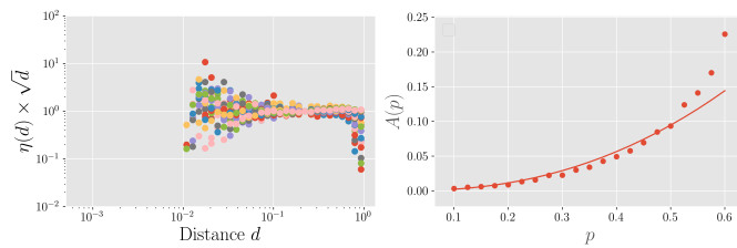
FIG. 6: Average detour for the honeycomb lattice. (a) We show the quantity \eta(d)\sqrt{d} versus d normalized by its value at d = 0.1 . The curves collapse onto a single one independent from d and the observed discrepancies for d close to 1 and d small come from finite-size effects. (b) The collapse suggest a form \eta(d) = A(p)d^{-1/2} , and a power law fit gives A(p) \sim p^\gamma with \gamma \approx 2.3 ( R^2 = 0.94 ). We, however, observe discrepancies at large p .
