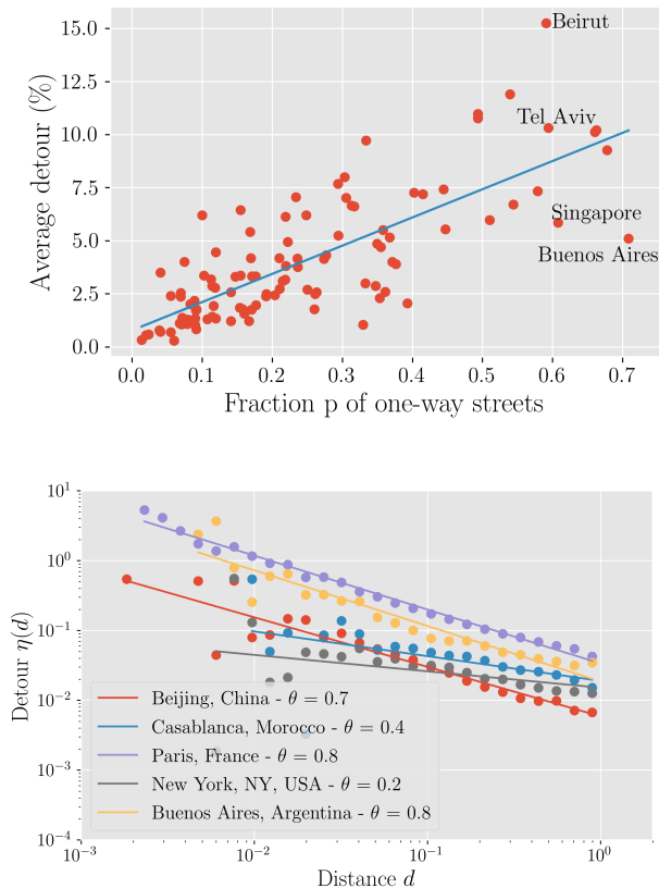
FIG. 2: (a) Distribution of the average detour (%) as a function of fraction p of one-way streets for 146 world cities ( R^2 = 0.59 ). (b) For five selected cities in the world, we plot the average detour \eta(d) due to one-way streets for a trip of distance d as a function of d (normalized by the maximum distance obtained for each city). The detour can be fitted by a power \eta(d) \sim d^{-\theta} . We find that \theta differs from one city to another and ranges roughly from 0.2 to 0.8. In particular, small exponent values (such as in the case of NYC) might be correlated with the presence of very long one-way streets leading to a large detour even at very large spatial scales. We have R^2 = 0.87 for Beijing, R^2 = 0.25 for Casablanca, R^2 = 0.99 for Paris, R^2 = 0.12 for NYC and R^2 = 0.90 for Buenos Aires.
