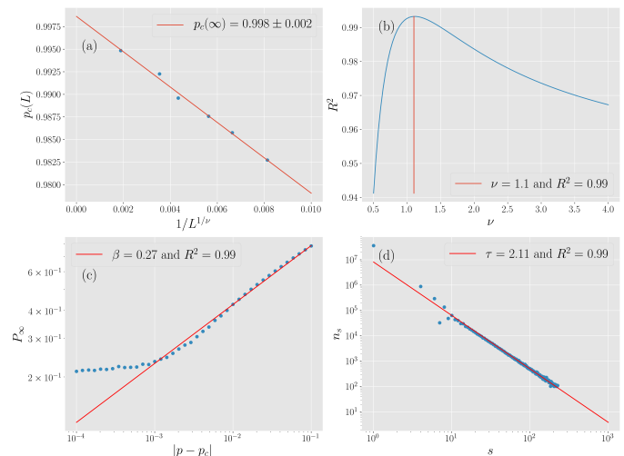
FIG. 9: (a) The percolation threshold for an infinite square lattice is calculated as an extrapolation for various finite-size lattices of side size ranging from L = 100 to L = 1000 . We find p_c = 0.998 \pm 0.002 . (b) The regression of the finite-size percolation threshold as a function of the linear size also gives the critical exponent \nu , and we obtain \nu = 1.1 \pm 0.2 . (c) Below criticality, the behavior of P_\infty with |p - p_c| gives the exponent \beta = 0.26 . (d) At criticality, the number of clusters of sizes s scales as a power-law of the size with critical exponent \tau and we find \tau = 2.14 \pm 0.05 .
