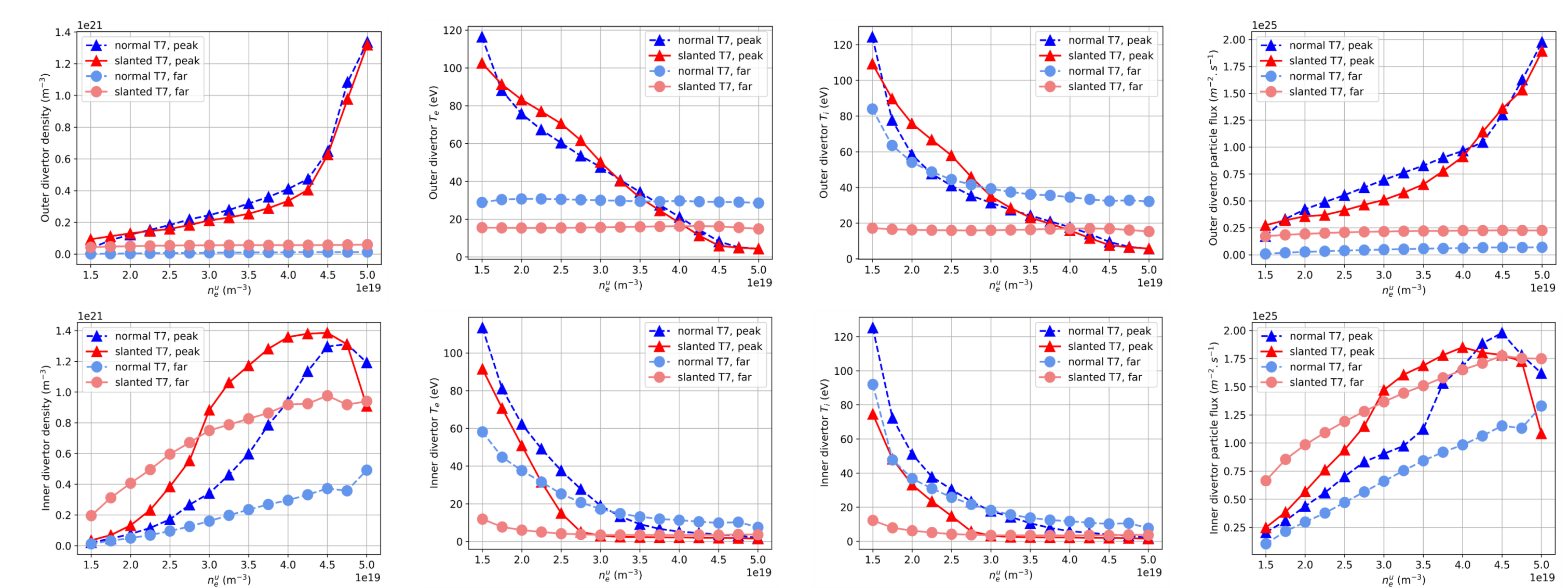
Fig. 8: Target conditions as a function of upstream density n_e^u . Top: outer divertor; bottom: inner divertor. Blue dashed lines = real T7, red full lines = slanted T7. Triangles = peak value at the strike point; circles = far SOL value.
