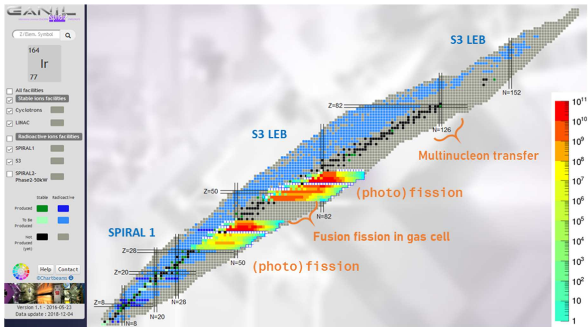
Figure VI.1. RIBs available from the existing SPIRAL 1 and the soon-to-be commissioned S3-LEB facility (in blue) and regions that would be populated thanks to fission and MNT reactions in the production building proposed here (in color plot and orange).
