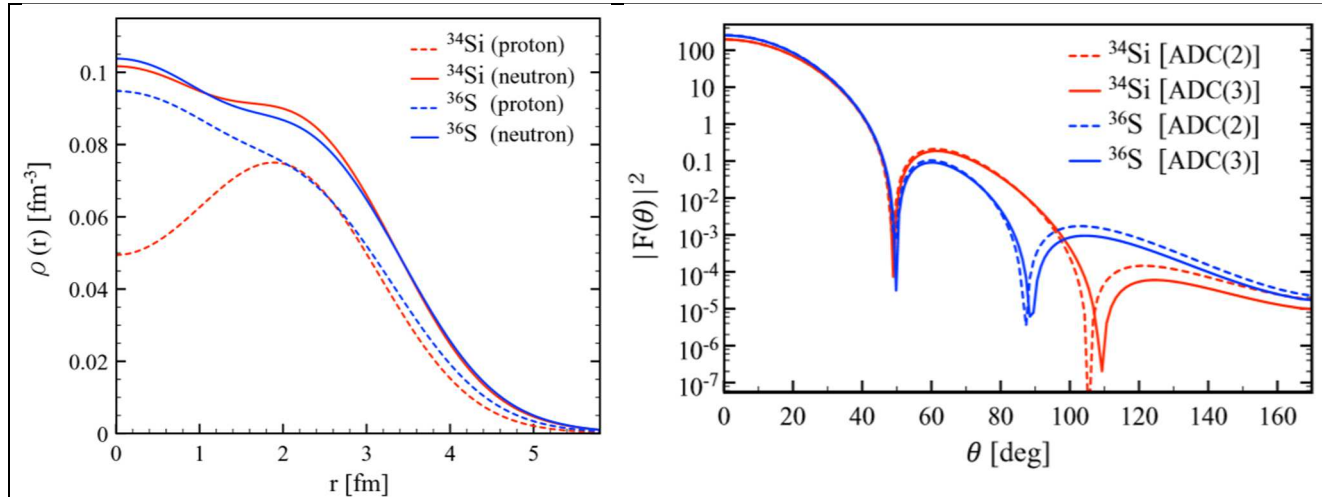
Figure I.2.1. Figures from [ Th34Siab ]. (Left) Ab initio calculations of point charge and neutron densities for ^{34}\text{Si} and ^{36}\text{S} isotopes. (Right) Angular dependence of the form factor obtained for 300 MeV electron scattering on ^{34}\text{Si} and ^{36}\text{S} . (Results from two computation techniques ADC(2) and ADC(3) are displayed).
