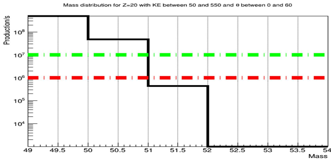
Figure 1. Estimated counts/s for different neutron-rich Ca isotopes (in black), obtained from using a 10 puA ^{48}\text{Ca} beam impinging on a 1 mg/cm 2 ^{238}\text{U} target. Estimation obtained using ref [1] and [2]. The green and red dash-dotted lines show the 10 7 counts/s and 10 6 counts/s limits respectively.
