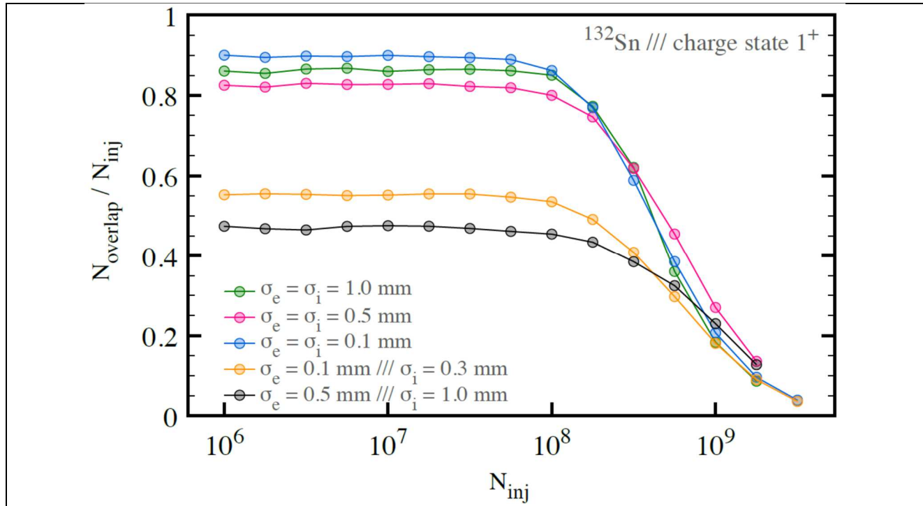
Figure III.4.4. Simulated number of ^{132}\text{Sn}^{1+} ions overlapping with the electron beam after injection ( t \sim 0.5 ms) for different values of electron beam \sigma_e and injected ion beam \sigma_i . An electron current of 200 mA and a trap length of 10 cm were used. In all cases a saturation appears close to the maximal theoretical value (for a number of ions compensating the electron space charge), N_{\text{overlap}}^{\text{max}} = 4 \cdot 10^8 for these conditions. The simulations were performed using WARP (see Appendix B for details).
