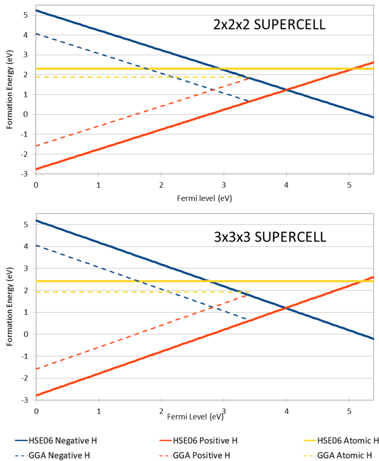
Figure 1: Formation energies (see Eq.1) of interstitial hydrogen as a function of Fermi level. Solid (resp. dotted) lines are for HSE06 (resp GGA) calculations. The x scale goes from the top of the valence band to the bottom of the conduction band as calculated by HSE06 functional. The dotted lines stop at the top of the GGA conduction band.
