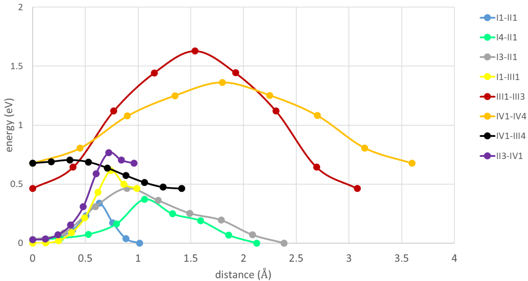
Figure 5: migration paths for H^+ protons in mZrO_2 . The colour scheme is consistent with the one of dotted lines in figure 3.
