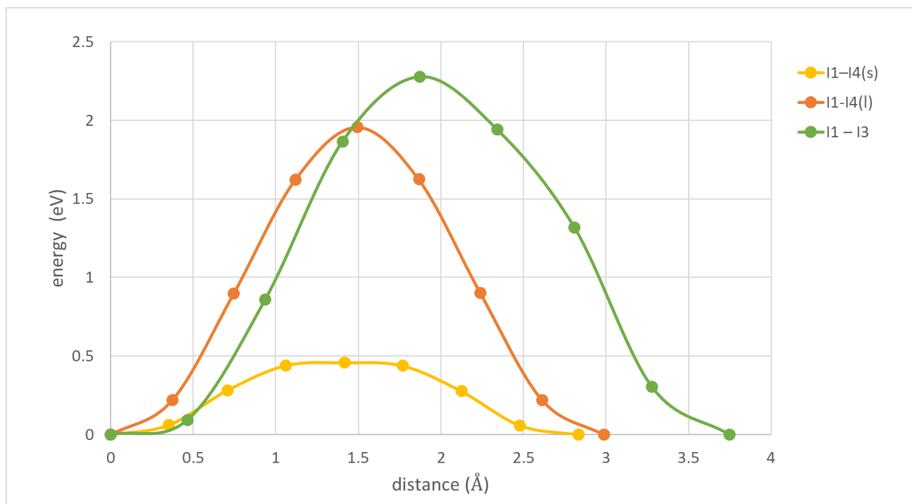
Figure 4: migration paths for H - hydride ions in mZrO 2 . The colour scheme is consistent with the one of dotted lines in figure 2.
