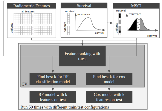
Fig. 1: Steps for features selection and survival prediction
