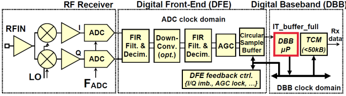
Fig. 1: Simplified architecture of software-defined RF receiver (reproduced from [9])
