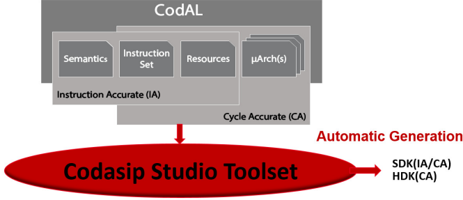
Fig. 9: CodaSip Studio [38]
