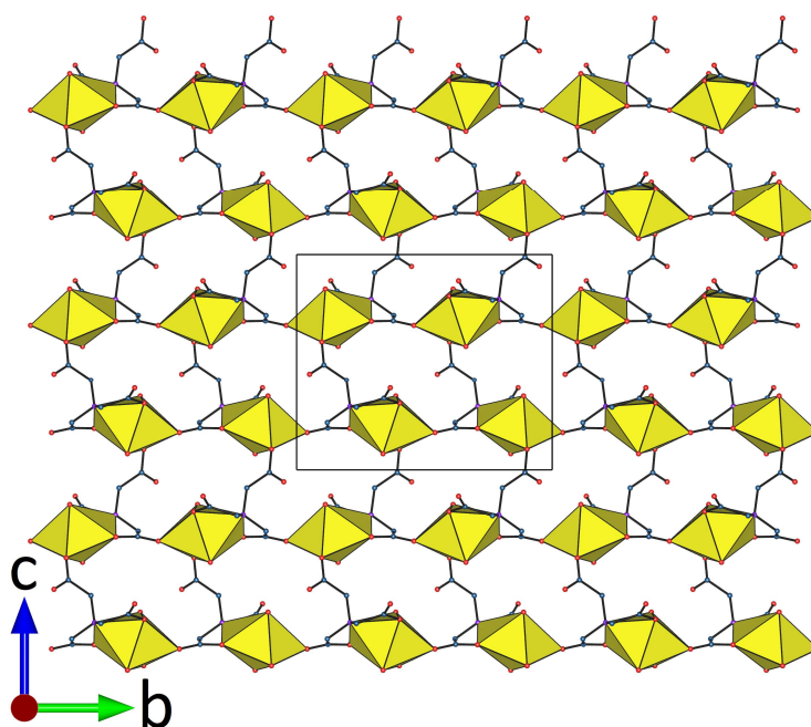
Fig. 6 View of the honeycomb-type network in 3 .
