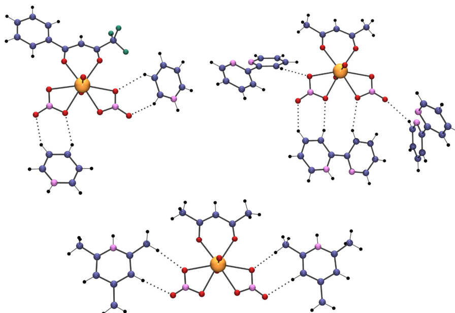
Fig. 4 CH...O interactions (dotted lines) in [UO 2 (diketonate)(NO 3 ) 2 ] - anions. (NH...O and NH...N interactions not shown).
