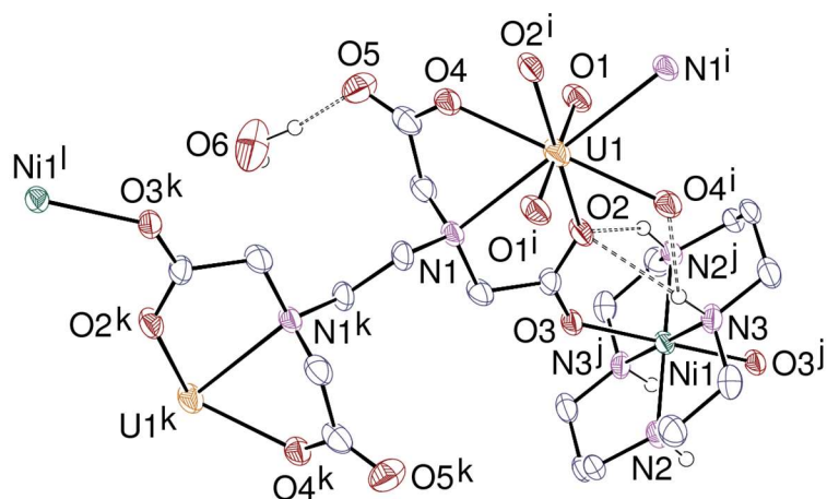
Fig. 7 View of [\text{Ni}(\text{cyclam})\text{UO}_2(\text{edta})]\cdot 2\text{H}_2\text{O} ( 4 ). Displacement ellipsoids are drawn at the 50% probability level. Carbon-bound hydrogen atoms are omitted and hydrogen bonds are shown as dashed lines. Symmetry codes: i = 1 - x, 1 - y, 1 - z ; j = 1 - x, 1 - y, 2 - z ; k = 2 - x, 1 - y, 1 - z ; l = x + 1, y, z - 1 .
