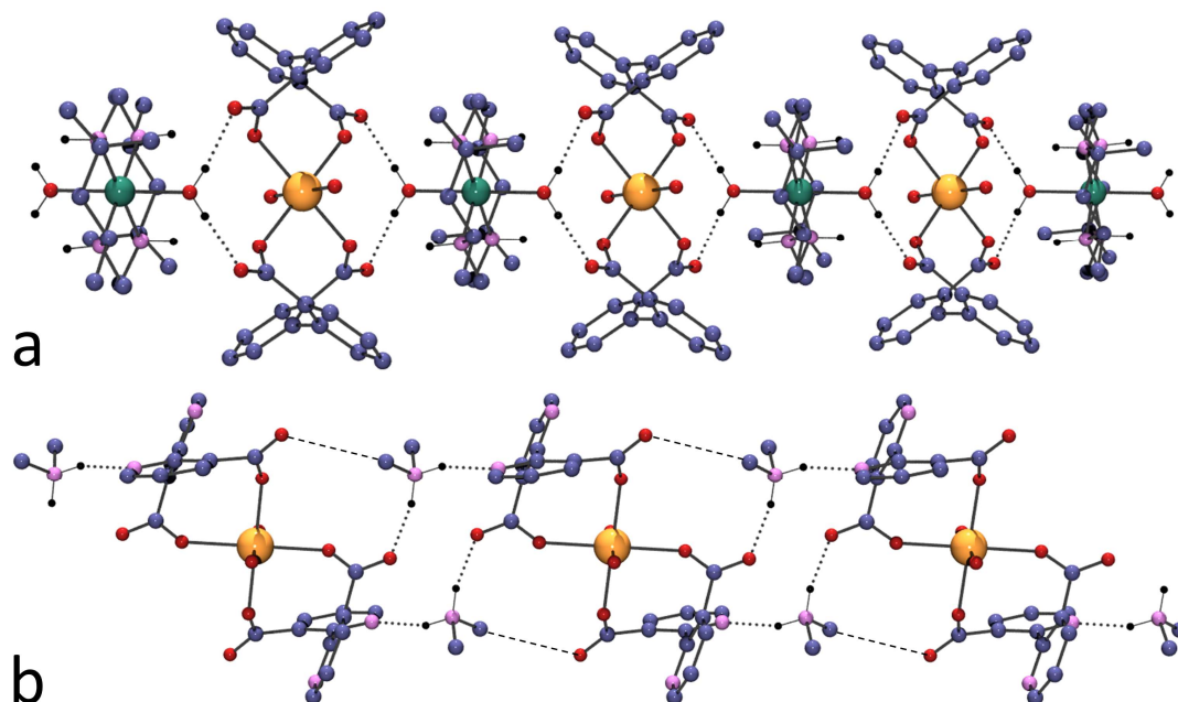
Fig. 2 Hydrogen-bonded chains in [\text{Ni}(\text{R,S-Me}_6\text{cyclam})(\text{H}_2\text{O})_2][\text{UO}_2(\text{dip})_2] (a) and in 1 (b). Carbon-bound hydrogen atoms are omitted; OH...O and NH...O/N hydrogen bonds are shown as dotted lines and CH...O bonds as dashed lines.
