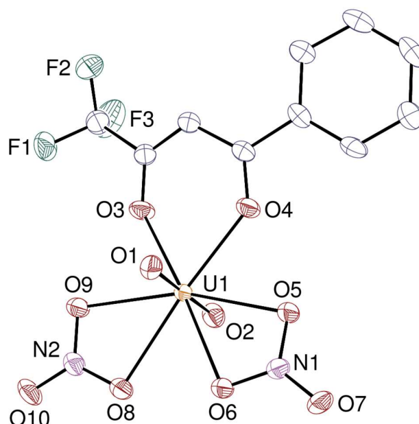
Fig. 3 View of the [UO 2 (tfbzac)(NO 3 ) 2 ] - anion in 2 . Displacement ellipsoids are drawn at the 50% probability level. Hydrogen atoms are omitted and the rotational disorder of the CF 3 group is not shown.
