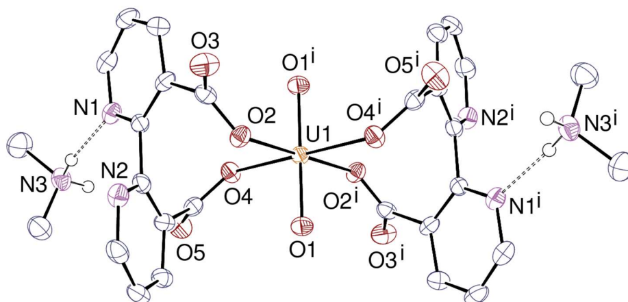
Fig. 1 View of [\text{H}_2\text{N}(\text{CH}_3)_2]_2[\text{UO}_2(\text{bpdc})_2] ( 1 ). Displacement ellipsoids are drawn at the 50% probability level. Carbon-bound hydrogen atoms are omitted and hydrogen bonds are shown as dashed lines. Symmetry code: i = 1 - x, 1 - y, 1 - z .
