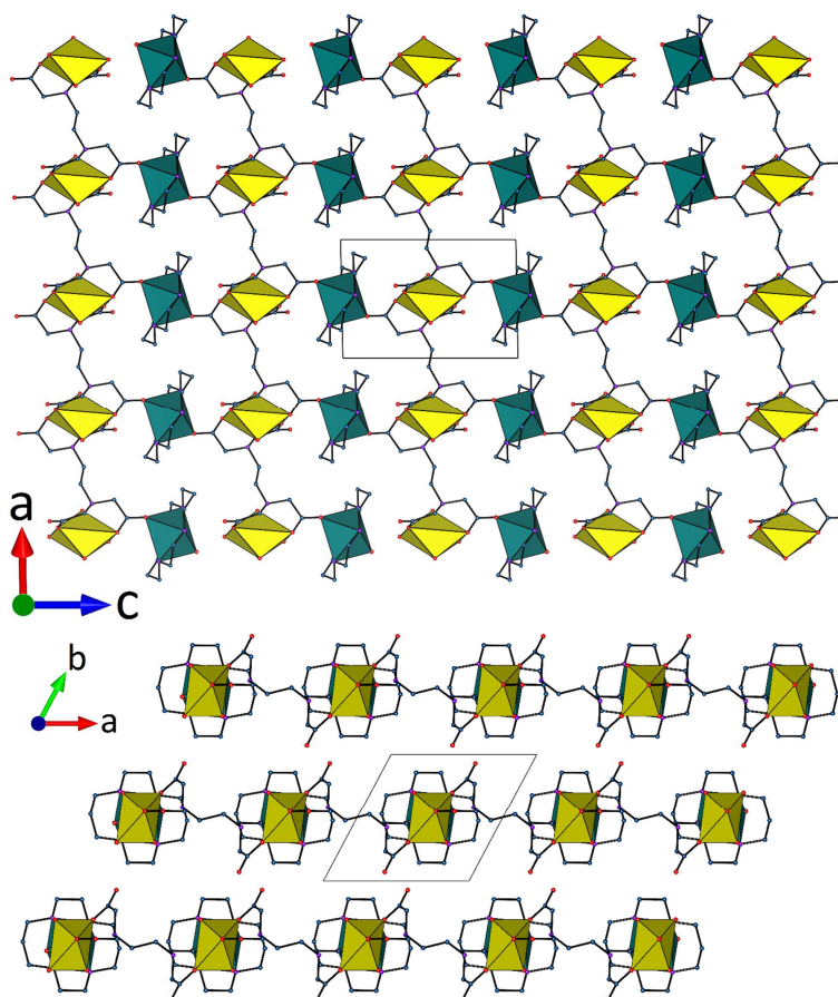
Fig. 8 Views of the diperiodic network (top) and of the packing of layers (bottom) in 4 . Hydrogen atoms and solvent molecules are omitted.
