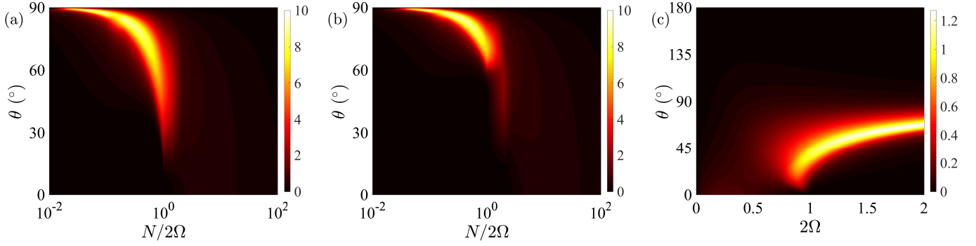
Fig. 19. (a,b) Contours of the maximum of the effective turbulent viscosity \max(v_{h,h}) in the parameter space (N/2\Omega, \theta) for Pe = \infty and (a) N = 1 , (b) N = 2 . (c) Contours of the maximum of the effective turbulent viscosity \max(v_{h,h}) in the parameter space (2\Omega, \theta) as Pe \rightarrow 0 .
