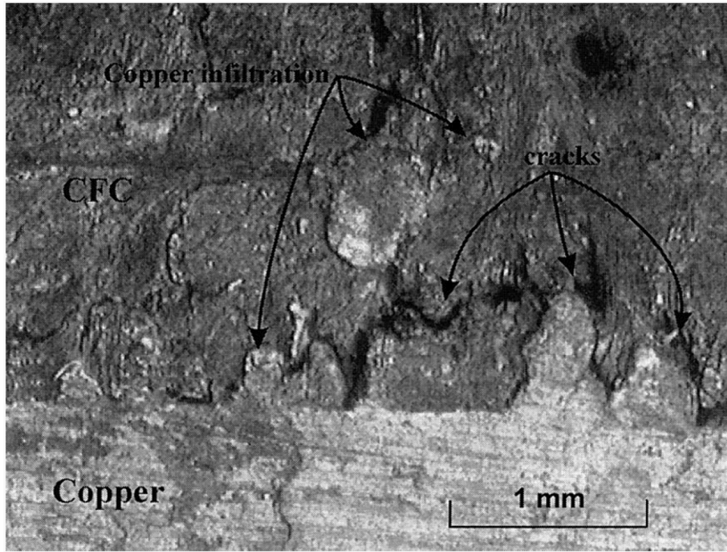
Figure 6 : Macrography of cracks in the CFC and at the interface CFC-copper.
