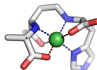
3D structure of staphylopin in complex with \text{Ni}^{2+} (ref. 44)
