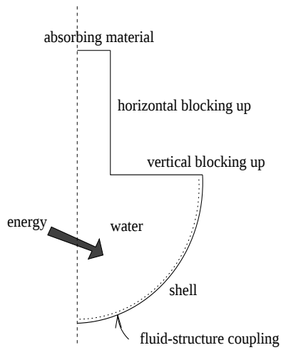
Figure 1: Accident scenario
